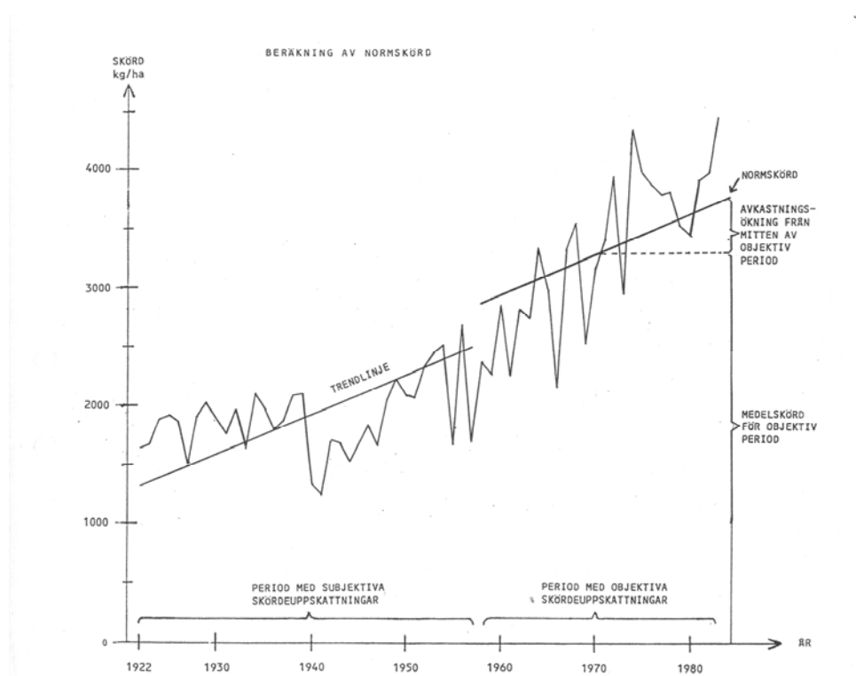
Fig. 2.8. Schematic description of the calculation procedure of the “standard yield” (source SCB, 1986).
