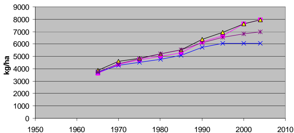
Fig. 2.4. Regional "standard yields" of winter wheat for every fifth year, as calculated by SCB. Squares are Kristianstad county, triangles are Malmöhus county, crosses are Halland county, and rhombs are average of "Götaland södra slättbygder".
