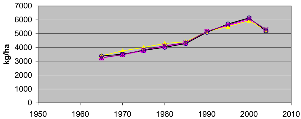
Fig. 2.5. Regional “standard yields” of winter wheat for every fifth year, as calculated by SCB. Squares are Stockholm county, triangles are Uppsala county, and rhombs are Södermanland county. Average values of “Svealands slättbygder” are similar to those of Stockholm county.
