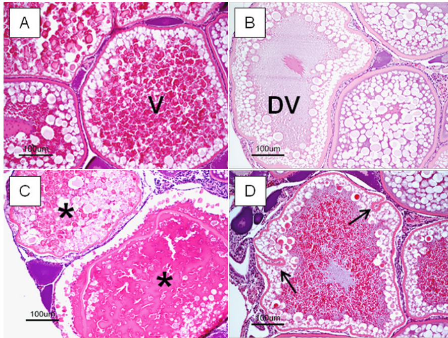
Figure 1. Light micrographs of ovaries from zebrafish exposed to control feed (A) or feed contaminated with 2,4,6-tribromophenol (B-D), showing different histopathological diagnoses. V = normal vitellogenic oocyte, DV = oocyte with decreased vitellogenesis, asterisk = atretic follicle, arrow = membrane folding. Haematoxylin-eosin staining.
