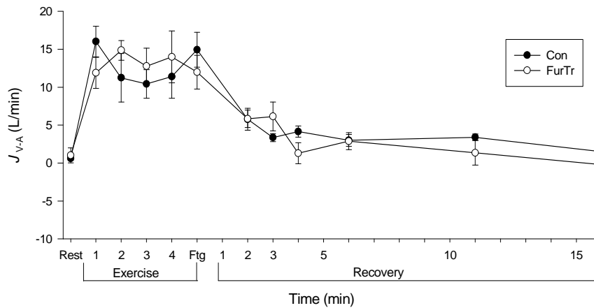
Figure 5. Fluid flux from/into the pulmonary vasculature ( J_{V-A} ) at rest, during exercise and recovery. Values are means \pm SE ( n=6 ). Ftg: fatigue. Positive values indicate decrease of J_{V-A} across the lung. Negative value indicate increase of J_{V-A} across the lung.
