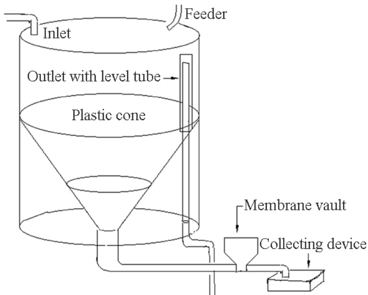
Figure 2. Schematic drawing of the experimental tanks. The tanks were built from cylindrical, dark green plastic tanks. Inside each tank was a plastic cone connected to a hole in the tank bottom, creating a space (approximately 55 l) with tilting walls. An automatic point source feeder was placed above each tank. The water inlet was placed on one side of each tank, and the water outlet (by a level tube) was placed on the other side. Feed waste and faeces were automatically evacuated from the tanks daily using timer controlled, air pressure driven membrane vaults and the effluents were collected in a mesh collecting device, allowing for excess water to run off but leaving the solid materials in the collecting device.
