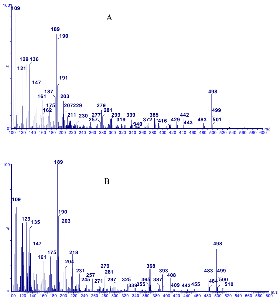
Figure 6. Full scan mass spectra of two 4,4'-dimethylsterols present exclusively in hazelnut oil. A) compound X; B) lupeol.
