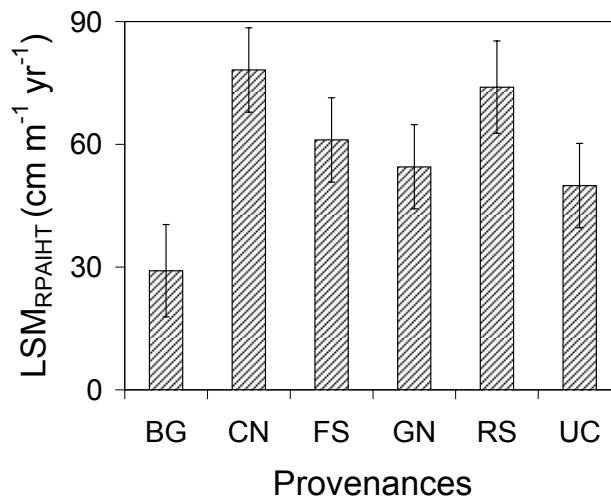
Figure 5. Least square means of relative periodic annual increment in height ( LSM_{RPAIHT} ) for various provenances of Casuarina cunninghamiana grown for 3.5 years after establishment at Halhale and Merhano on Eritrean highland. BG, CN, FS, GN, RS and UC are ‘Bega’, ‘Coonabarabran’, ‘Flag Stone’, ‘Glen Innes’, ‘Rollingstone’ and ‘Uriarra Crossing’ provenances of the species, respectively.
