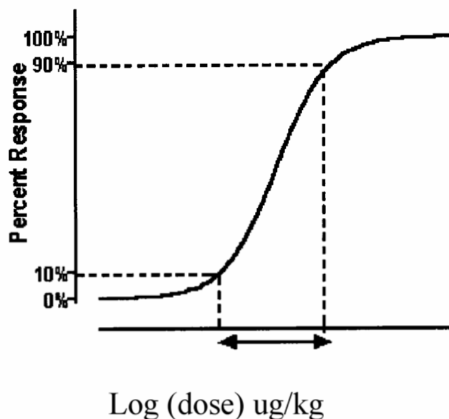
Figure 4. Illustration of the concentration plateau attained in the verification of LODs
