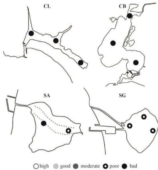
Figure 3. Classification of water quality at the sampling stations, based on the MPI.
