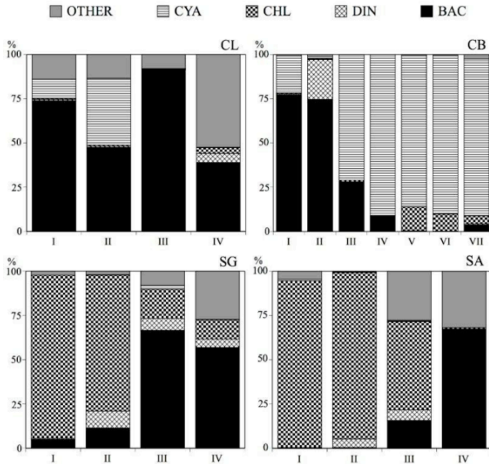
Figure 2. Mean annual density of phytoplankton classes in the four lagoons studied.
