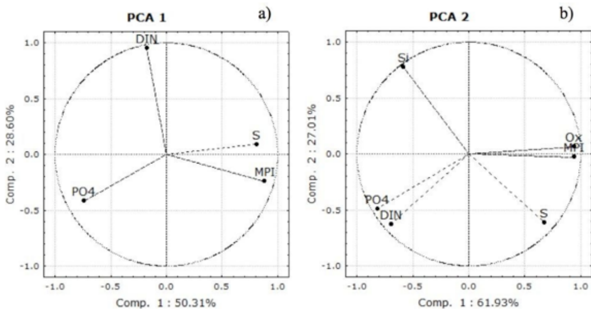
Figure 4. a) PCA1, comparing the four Sardinian lagoons and the reference site. b) PCA2, comparing CL, CB and the reference site. The variance of each component is reported in the axis title.
