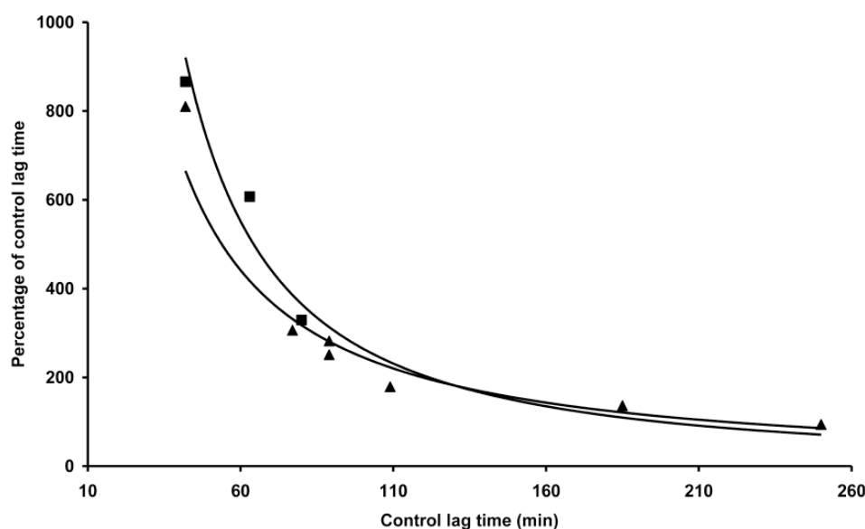
Fig. (3). \text{Cu}^{2+} catalysed LDL peroxidation: influence of \text{Cu}^{2+} concentration on coffee effect.
