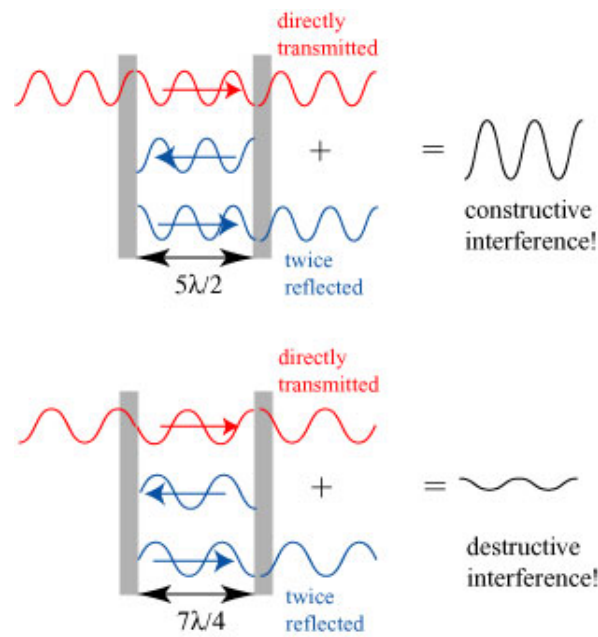
Figure 3.1: Interference within the Fabry-Pèrot cavity. Source: SkullsInTheStars 2008
