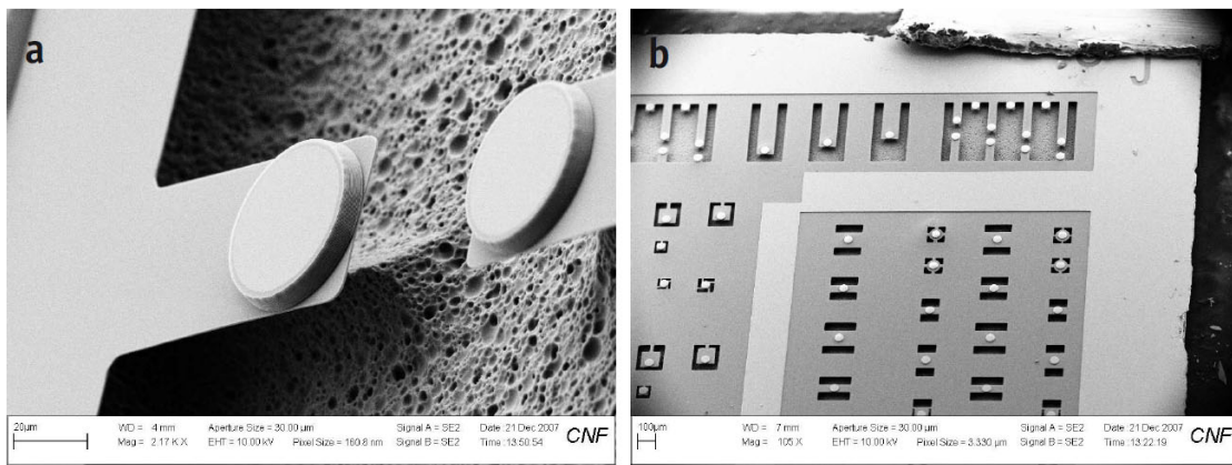
Figure 3.2: a: Scanning electron microscope (SEM) image of a pair of cantilevers ( \varnothing_{mirror} = 20\mu m ).
