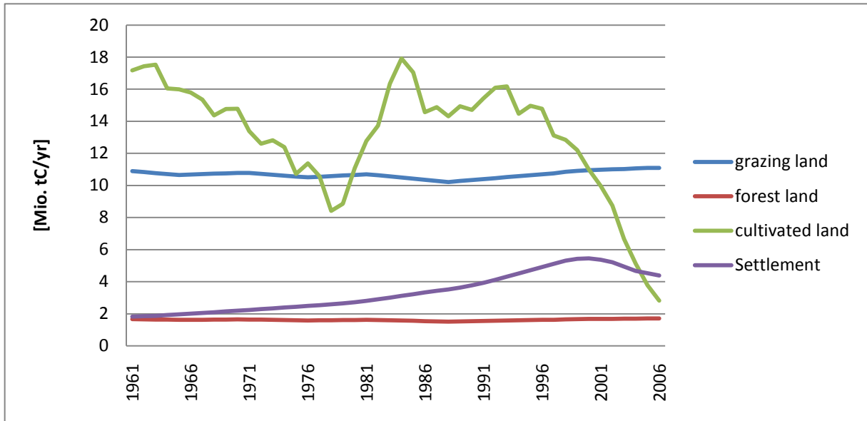
Figure 29: aNPP ic from 1961 to 2006 in 5-year means
