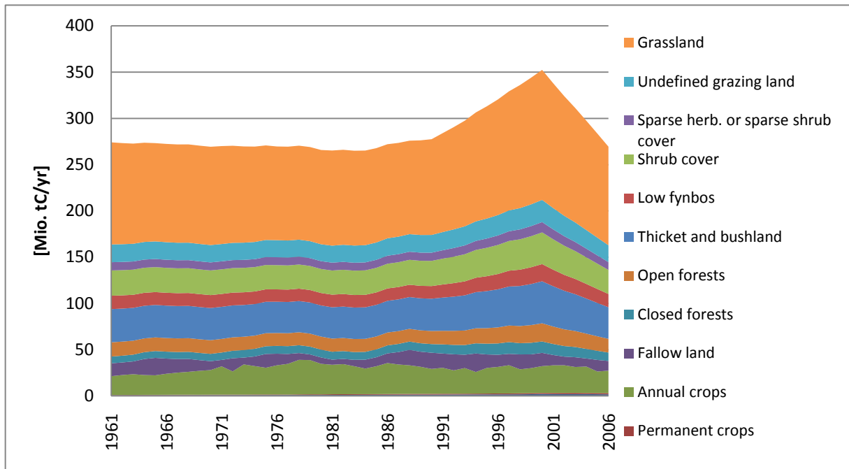
Figure 9: aNPP act in the RSA from 1961 to 2006, split into the single land cover classes
