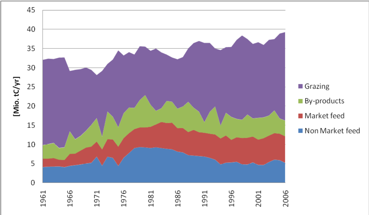
Figure 18: Feed supply for livestock species from 1961 to 2006
