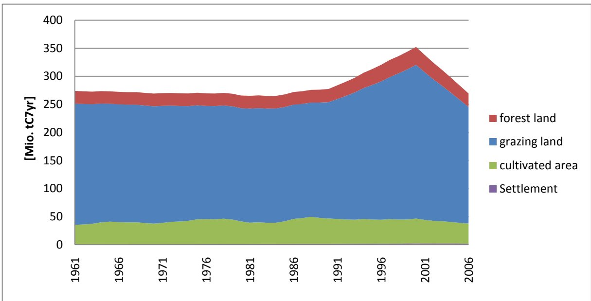
Figure 28: aNPP act from 1961 to 2006 in 5-year means
