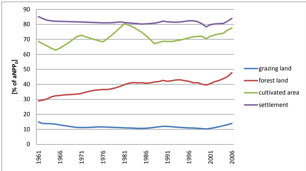
Figure 33: aHANPP as percentage of aNPP 0 from 1961 to 2006
