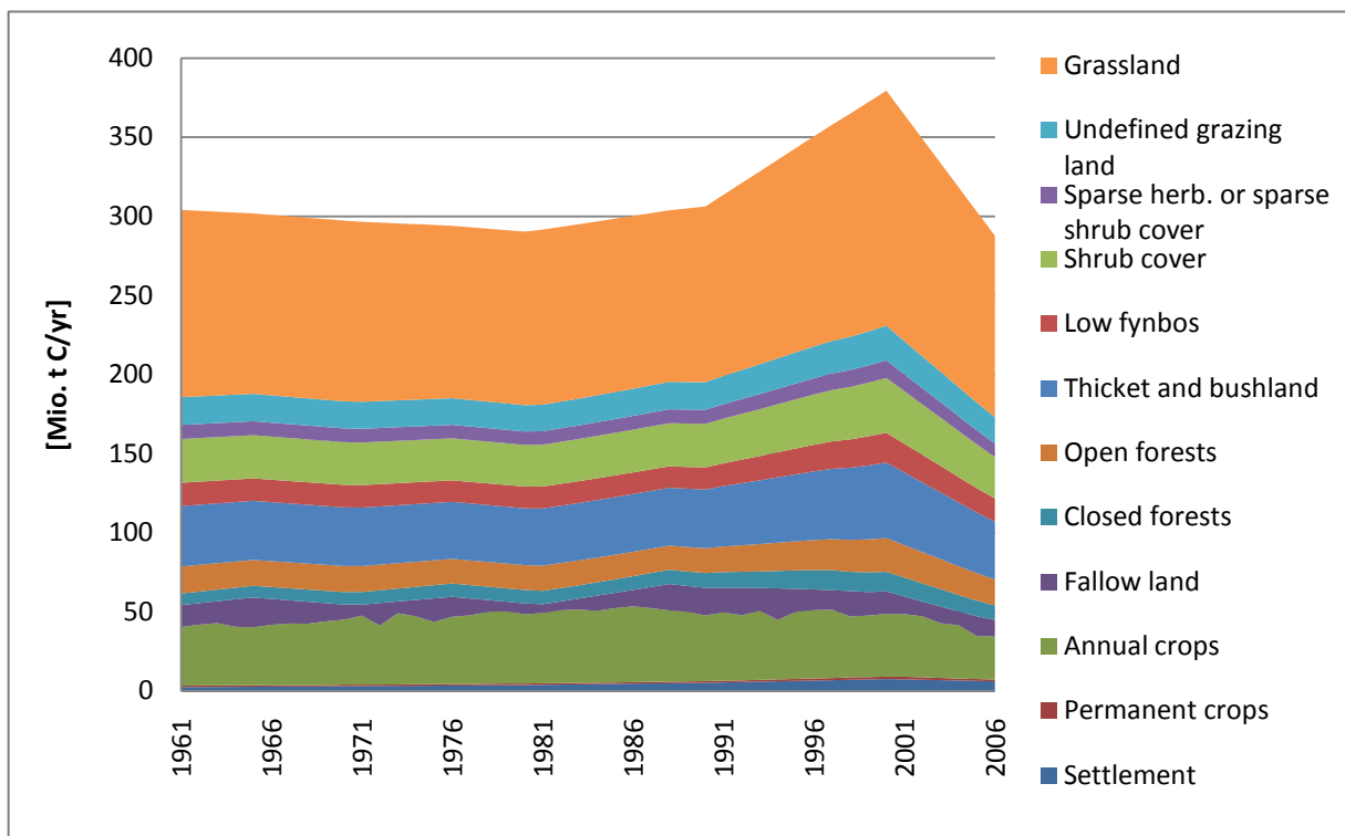
Figure 7: Trend in aNPP 0 for the RSA from 1961 to 2006, split into land cover classes Source: Haberl et al. (2007), own estimations, see text
