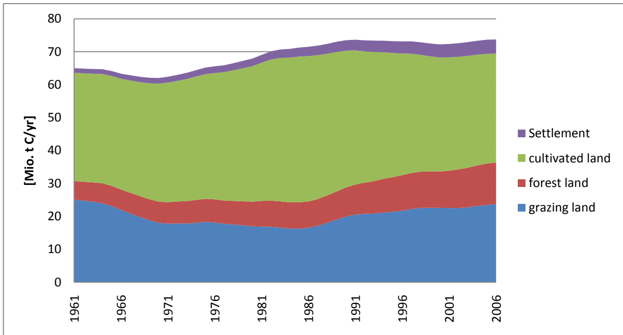
Figure 32: aHANPP development from 1961 to 2006 in 5-year means
