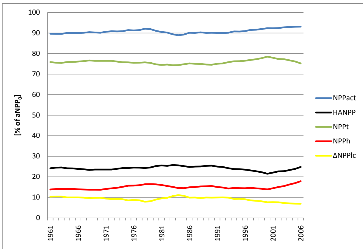
Figure 24: aNPP act , aHANPP, aNPP t , aNPP h , ΔaNPP ic as percentage of aNPP 0
