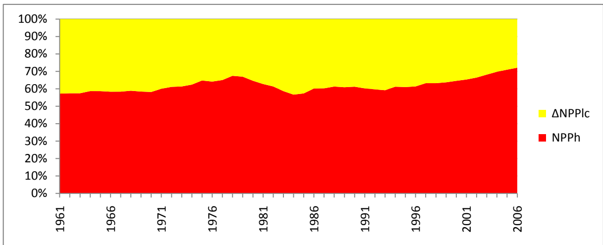
Figure 22: aNPP h and \Delta aNPP lc as percentage of aHANPP
