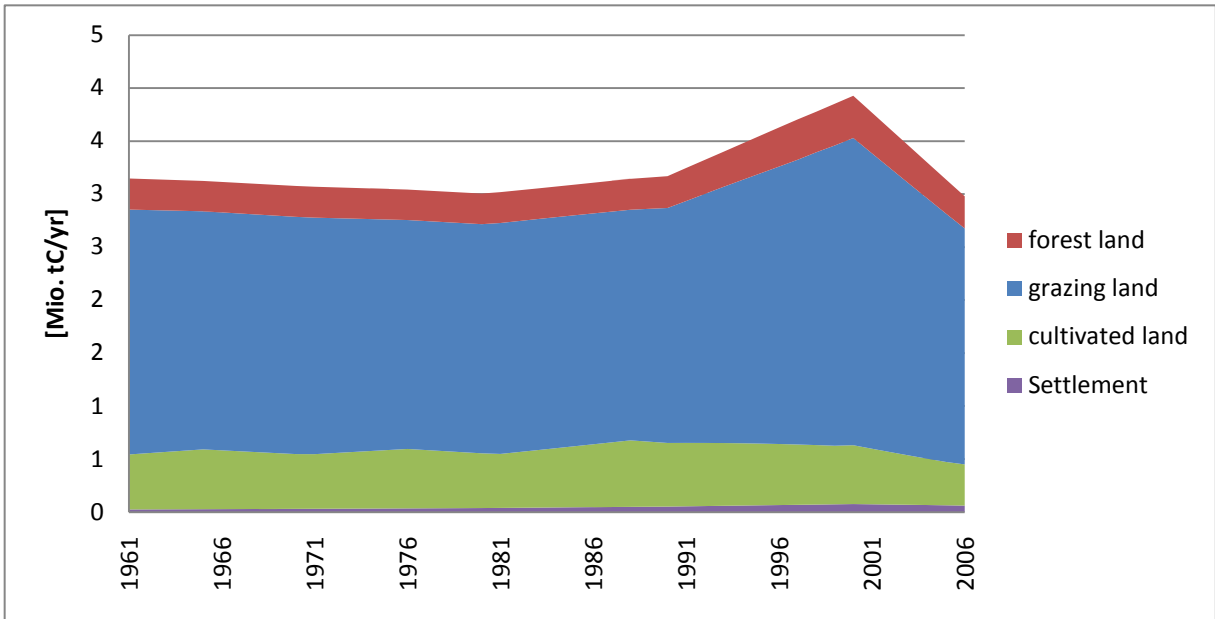
Figure 27: aNPP 0 from 1961 to 2006 in 5-year means
