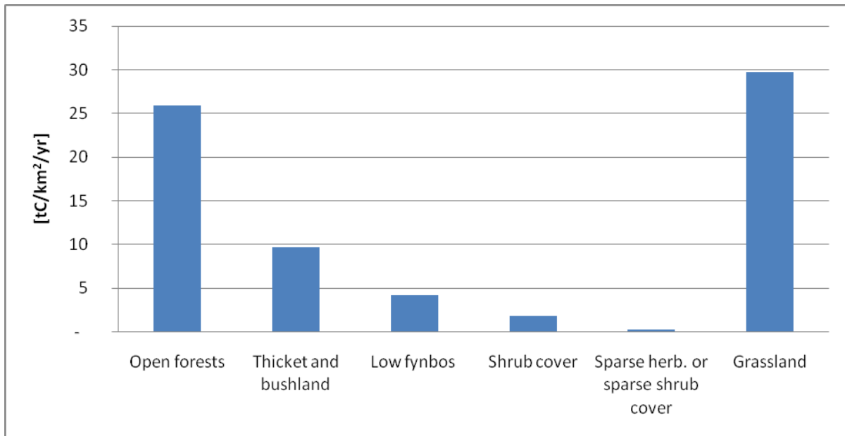
Figure 10: \Delta\text{aNPP}_{\text{lc}} for all land cover categories affected by land degradation in (constant value from 1961 to 2006)
