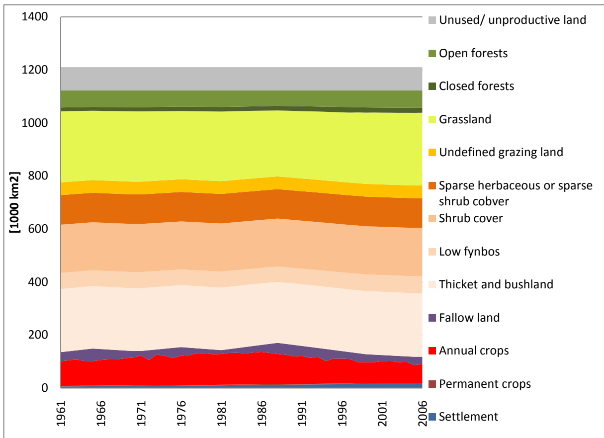
Figure 5: Land cover change in South Africa from 1961 to 2006
