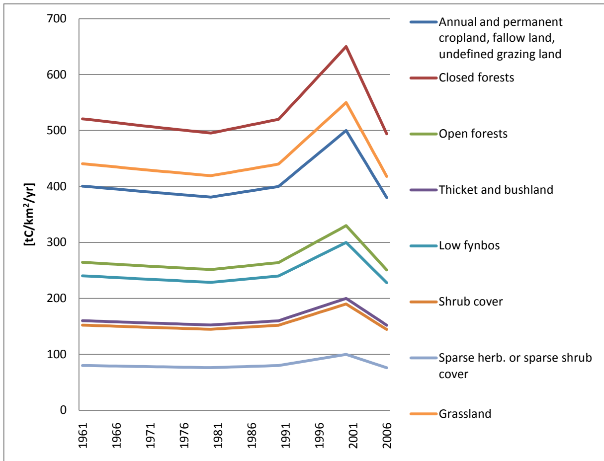
Figure 8: aNPP_0 for each land cover class
