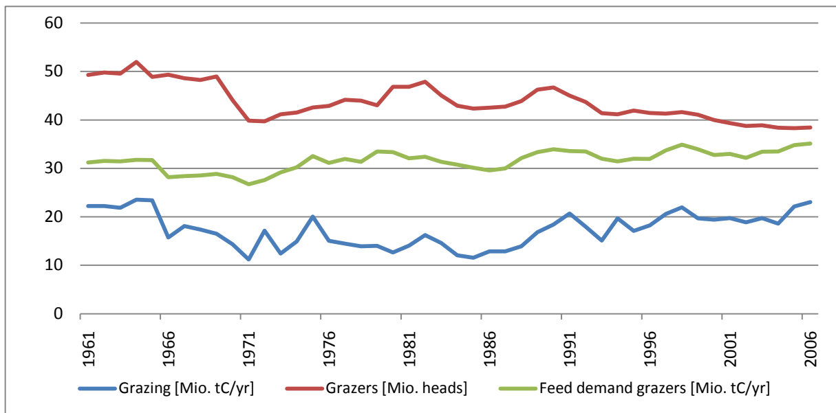
Figure 19: Grazing and its components in the RSA from 1961 to 2006
