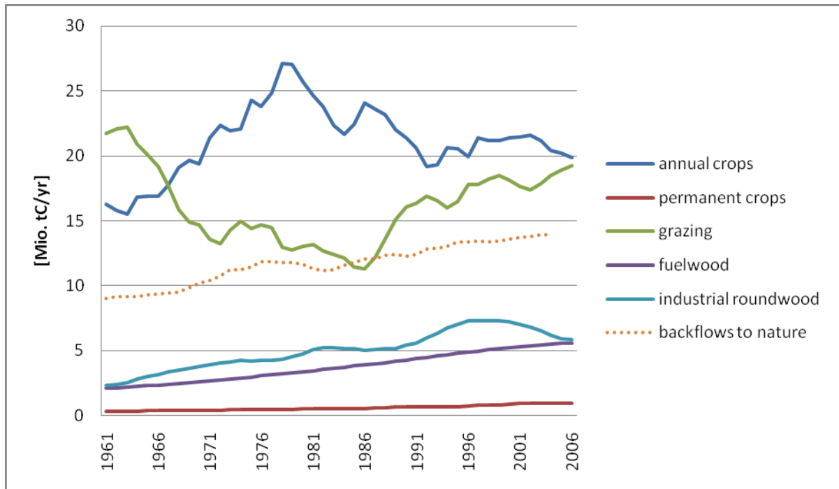
Figure 13: Development of aNPP h broken down to its components from 1961 to 2006
