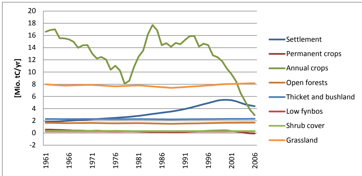
Figure 11: \Delta aNPP_{lc} from 1961 to 2006 for each land cover class
