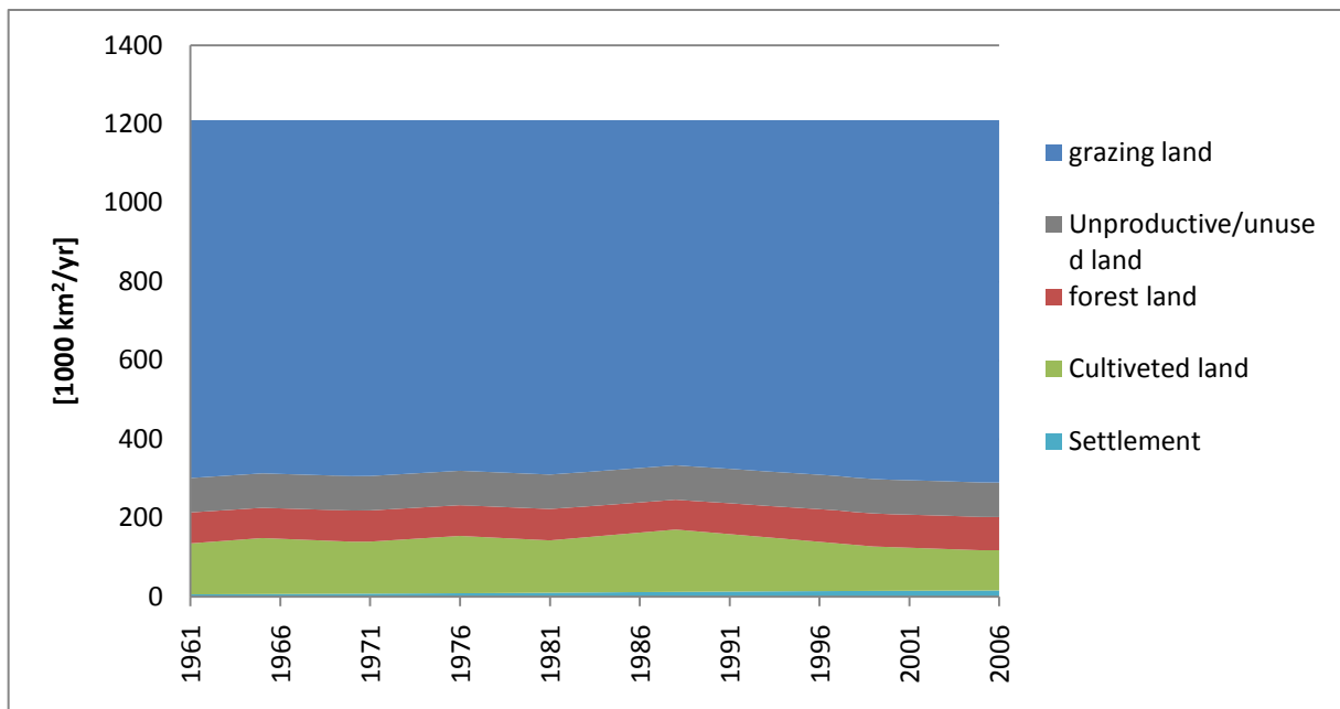
Figure 26: Land cover change from 1961 to 2006 in 5-year means
