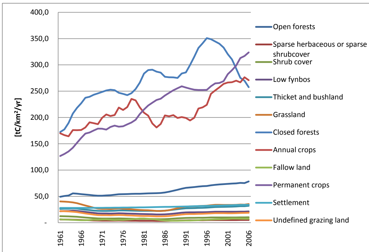
Figure 14: Harvest per km 2 land cover class from 1961 to 2006
