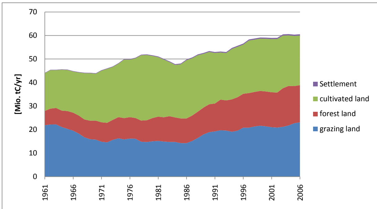
Figure 30: aNPP h from 1961 to 2006 in 5-year means
