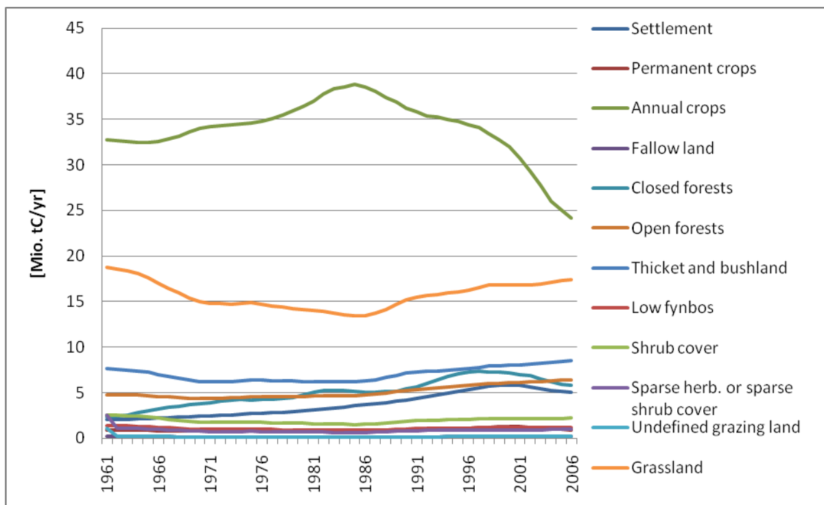
Figure 23: Development of aHANPP on land cover classes from 1961 until 2006 in 5-year means
