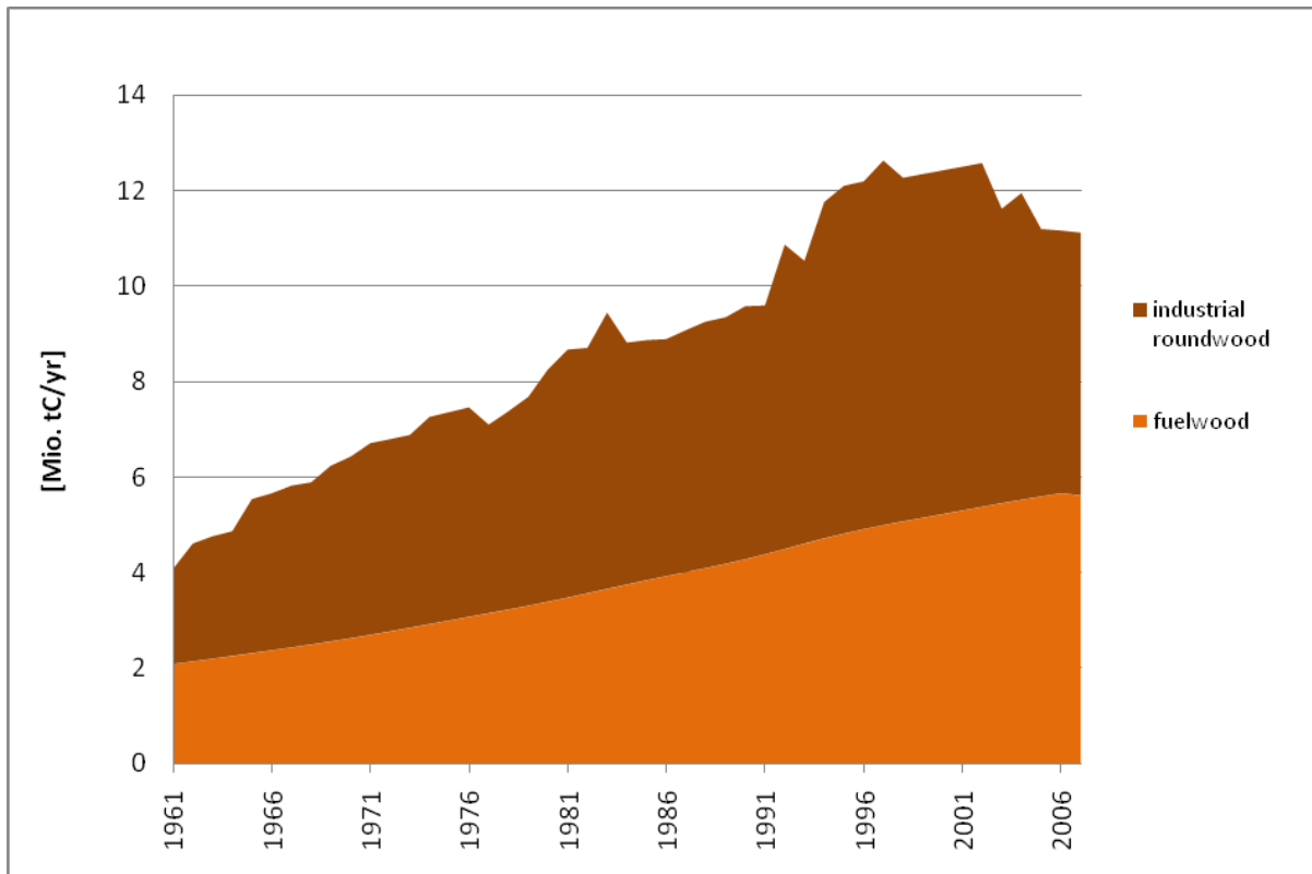
Figure 20:a NPP h of fuelwood and industrial roundwood
