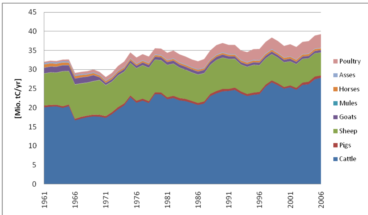
Figure 17: Feed demand for livestock species from 1961 to 2006 Sources: FAOSTAT, own calculations
