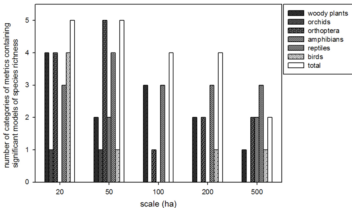
Figure B.2.1. Relations between landscape structure, organism groups and scale expressed by the number of categories of univariate models (out of the six categories "area", "shape", "contrast", "isolation", "texture", and "diversity") containing at least one model that relates significantly a landscape metric with species richness. While reptiles were still predictable considering the surrounding 500 ha, for the other taxa the performance of landscape metrics as indicators of species richness declined clearly at the larger scales.
