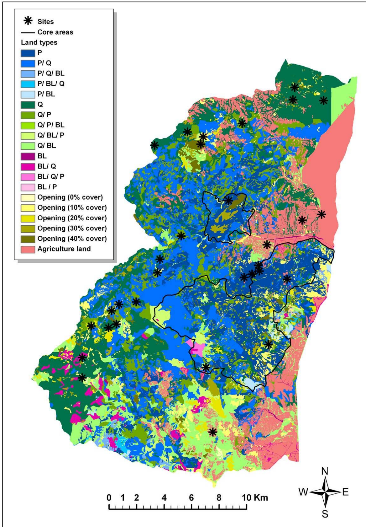
Appendix B.4.1. Vegetation map of the 20 landcover types in Dardia National Park and sites sampled. Forest types: P - pine , Q - oak, BL - broadleaved
