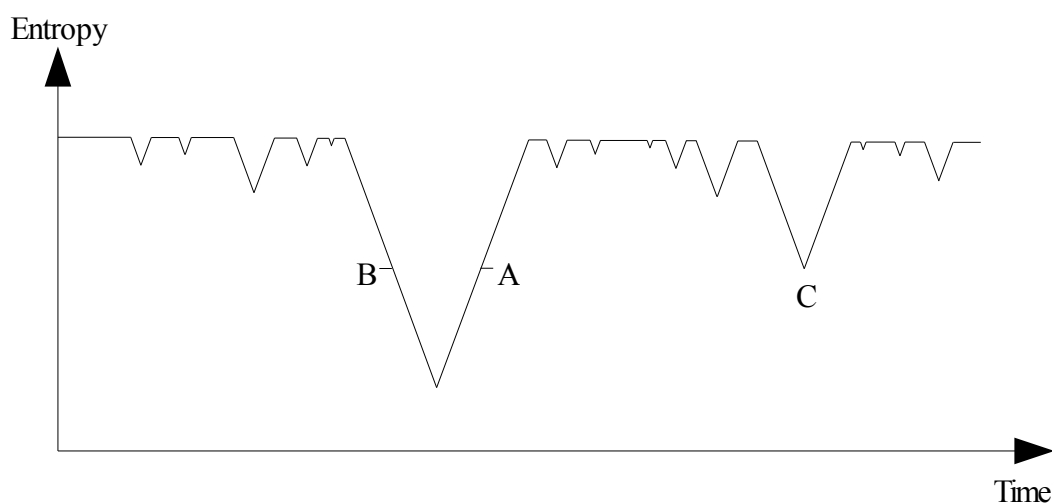
Illustration 5: Boltzmann's Entropy Curve
