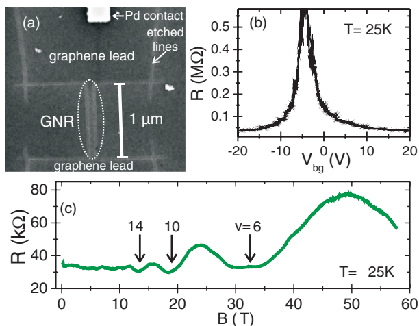
FIG. 1. (Color online) (a) Scanning electron microscope image of a typical sample. The length of the GNRs is 1\ \mu\text{m} , the width is 70\ \text{nm} . In the upper part of the image a palladium contact is visible. (b) Two-terminal resistance as a function of V_{\text{bg}} at T = 25\ \text{K} and zero magnetic field. (c) Magnetoresistance trace at V_{\text{bg}} = -20\ \text{V} , showing quantum Hall features at \nu = 6, 10 , and 14 .
