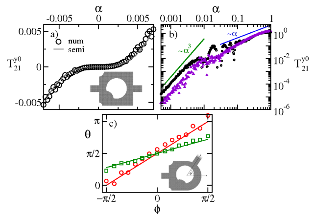
Figure 1: (Color online) Spin-dependent transmission coefficients \mathcal{T}_{21}^{y0} , Eq. (4), for (a) weak and (b) extended range of SO coupling showing the crossover from cubic (green line) to linear (blue line) behavior for the two-terminal chaotic quantum dot shown in the inset of panel (a). (c) Spin current polarization angle \theta = \arctan(\mathcal{T}_{21}^{y0}/\mathcal{T}_{21}^{x0}) , for the system shown in the inset, where the right lead encloses an angle of \phi with the x -axis in the linear (cubes) and the cubic (circles) regimes.
