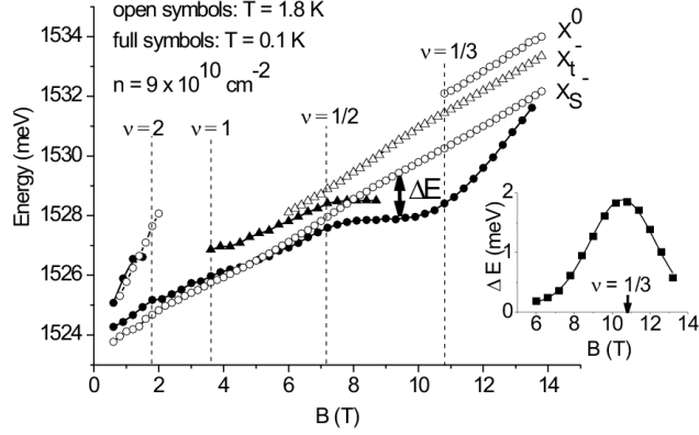
Fig. 7. Experimentally observed mode positions at T = 1.8 K (open symbols) and T = 0.1 K (solid symbols). The inset shows the anomaly \Delta E versus magnetic field.
