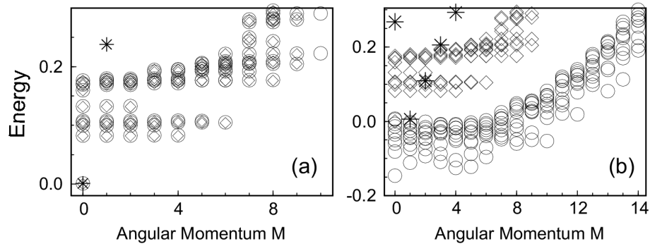
Fig. 8. Energy (in units of Coulomb energy) versus the azimuthal rotational quantum number M for an isolated quantum dot (*), a two-dimensional electron liquid ( \diamond ), and a qd-liquid ( \circ ). The QD of the qd-liquid either contains (1e,h) [in (a)], or (2e,h) [in (b)].
