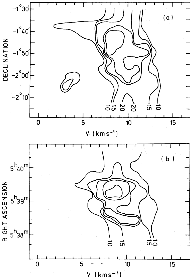
Figure 1. (a) Declination-velocity map of the ^{12}\text{CO} line intensity in NGC 2024. The map was made along constant RA = 05 h 39 m 14 s . The lowest contour level is at 10 K, with intervals of 5 K. The low-velocity features with V < 6 km/s are probably due to noise or interference spikes on several bad channels. (b) Right Ascension-velocity map along constant dec = -01° 44' 57". Other details as in Fig. 1(a).
