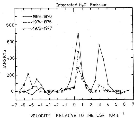
Figure 12. A comparison of the average spectra over the periods 1974-76 and 1976-77 with that of Sullivan (1973) over the period 1969 April-1970 March for W75S.
