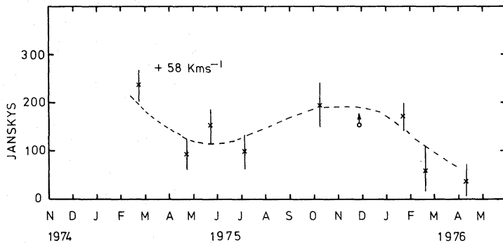
Figure 6. Intensity variation of the +58 km/s component in W33B.
