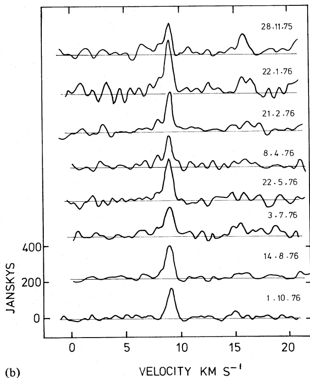
Figure 3. Spectra of S255 with velocity resolution 0.4 km/s.
