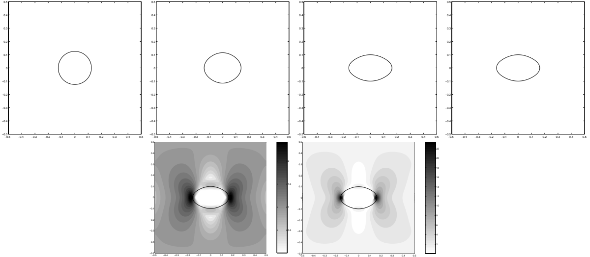
Figure 2: ( \underline{S} = \begin{pmatrix} 0 & 0 \\ 0 & 1 \end{pmatrix} , \Lambda = \frac{1}{5} , \gamma = \frac{1}{12\pi} ) Zero level sets for \Theta_\varepsilon(x, t) at times t = 0, 1.5 \times 10^{-4}, 1.5 \times 10^{-3}, 0.02 and elastic stress field and elastic energy at time t=0.02 .
