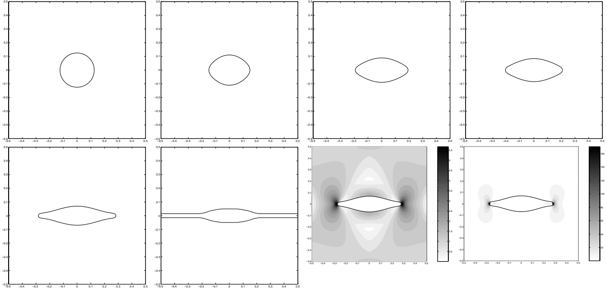
Figure 3: ( \underline{S} = \begin{pmatrix} 0 & 0 \\ 0 & 1 \end{pmatrix} , \Lambda = \frac{1}{5} , \gamma = \frac{1}{24\pi} ) Zero level sets for \Theta_\epsilon(x, t) at times t = 0, 1.5 \times 10^{-4}, 1.5 \times 10^{-3}, 3 \times 10^{-3}, 3.75 \times 10^{-3}, 5.25 \times 10^{-3} and elastic stress field and elastic energy at time t = 3.75 \times 10^{-3} .
