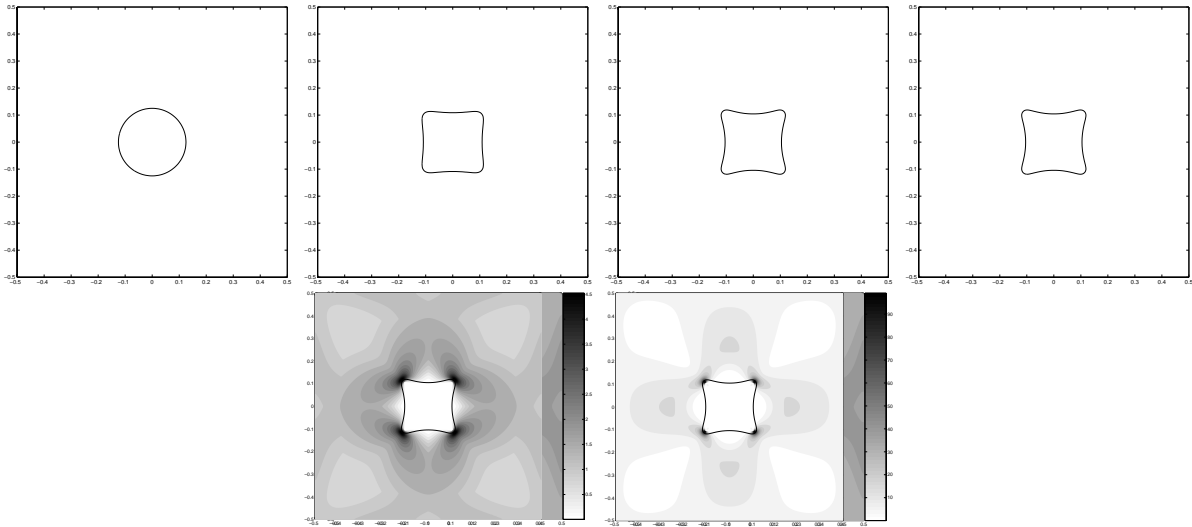
Figure 7: ( \underline{S} = \begin{pmatrix} 0 & 1 \\ 1 & 0 \end{pmatrix} , \Lambda = \frac{1}{5} , \gamma = \frac{1}{24\pi} ) Zero level sets for \Theta_\epsilon(x, t) at times t = 0, 1.5 \times 10^{-4}, 1.5 \times 10^{-3}, 0.02 and elastic stress field and elastic energy at time t=0.02 .
