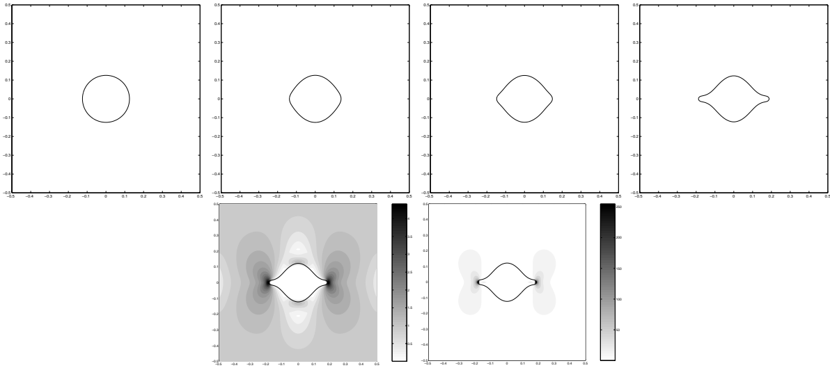
Figure 5: ( \underline{\underline{S}} = \begin{pmatrix} 0 & 0 \\ 0 & 1 \end{pmatrix} , \Lambda = \frac{1}{2} , \gamma = \frac{1}{24\pi} ) Zero level sets for \Theta_\varepsilon(x, t) at times t = 0, 3 \times 10^{-6}, 5 \times 10^{-5}, 10^{-5} and elastic stress field and elastic energy at time t=10^{-5} .
