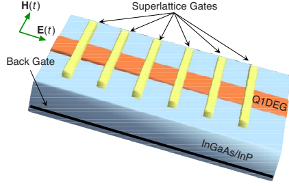
FIG. 1. (Color online) A 2DEG with RSOI of strength \alpha=9.94 \times 10^{-12} eV·m is obtained by a gate voltage applied to an InGaAs/InP heterostructure using the “back gate.” The electron effective mass is m=0.037m_0 with m_0 being the free electron mass and the effective gyromagnetic factor is g^*=-15 . A parabolic confinement of strength \hbar\omega_0=0.225 meV forms in the 2DEG a quasi-one-dimensional electron gas. The superlattice with period L=0.25 \mu\text{m} is shaped by the “superlattice gates” which create a symmetric periodic potential. The system is driven by a longitudinal electric field \mathbf{E}(t) and by a transverse magnetic field \mathbf{H}(t) which are time symmetric.
