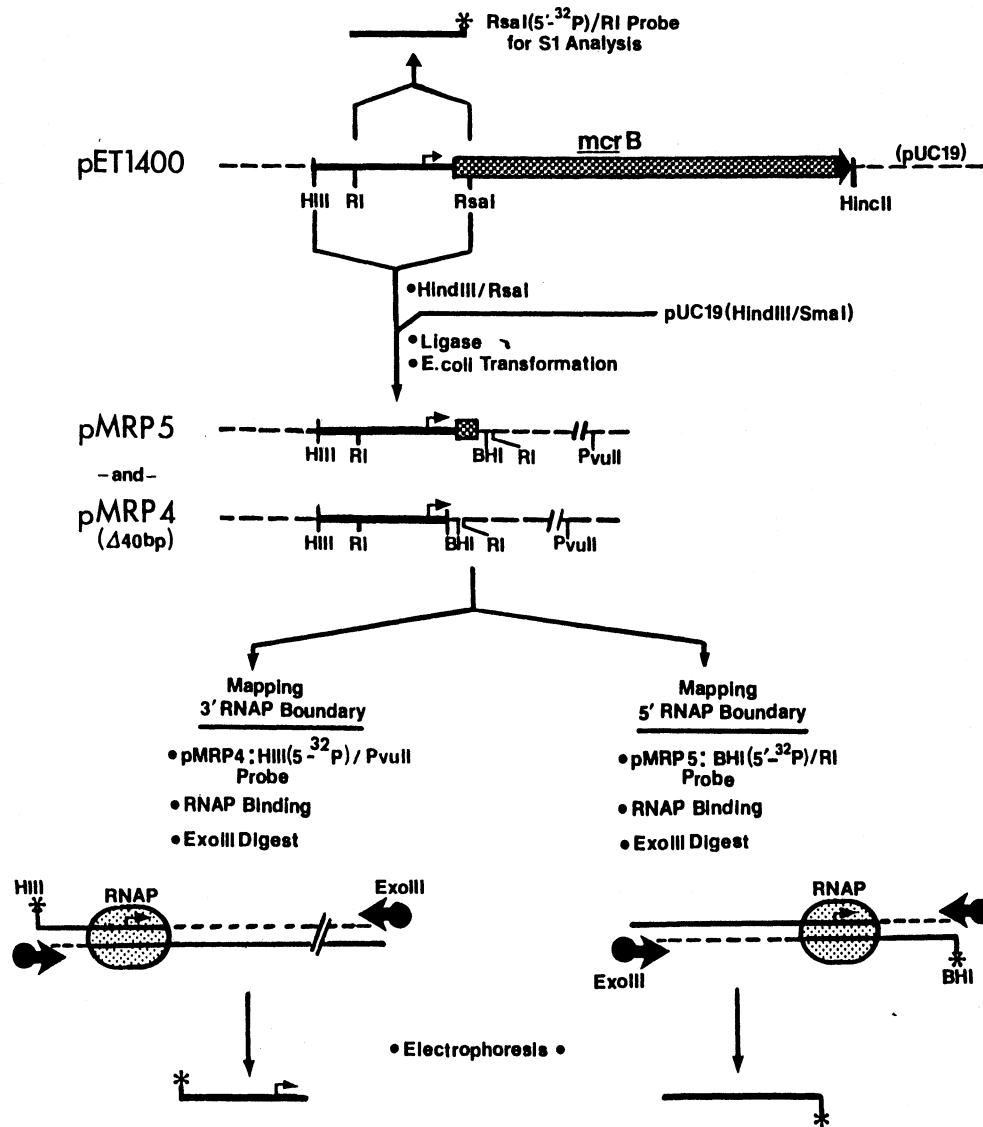
FIG. 1. Probes and experimental protocols used. Plasmid pET1400 contains part of the mcrB gene (hatched) and the intergenic region (solid line) upstream of the mcrB gene cloned in pUC19 (1, 10). Restriction fragments, 5' end labeled by means of polynucleotide kinase and [ \gamma - 32 P]ATP, were subsequently cleaved by restriction enzymes as indicated to obtain the single-end-labeled molecules used as probes. Locations of 32 P atoms are denoted by asterisks, and the in vivo initiation site and direction of transcription are indicated by the small rightward-pointing arrow. DNA which would be digested by ExoIII activity in the presence of RNAP is also indicated (---). Restriction sites are indicated by the standard abbreviations except for HindIII (HIII), EcoRI (RI), and BamHI (BHI). The sequence of the M. vannielii DNA shown has been published previously (1). Standard techniques were used for the in vitro DNA manipulations, S1 analysis, and ExoIII footprinting (4, 7, 10, 13).
