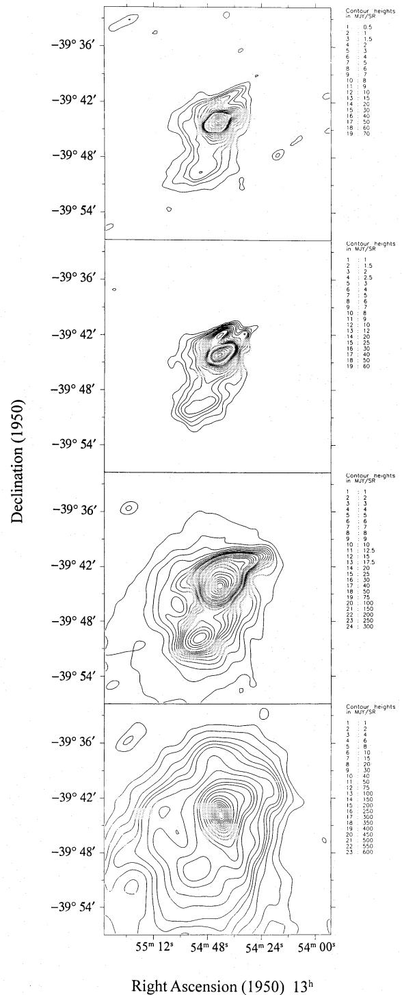
Fig. 3. IRAS maps using the HIRES processing algorithm. The four maps show the a) 12 \mu\text{m} , b) 25 \mu\text{m} , c) 60 \mu\text{m} and d) 100 \mu\text{m} bands respectively, and have beamsizes 78 \times 51'' , 120 \times 45'' , 96 \times 71'' and 101 \times 102'' respectively, with the major axes of the distribution at position angle 148^{\circ} , orthogonal to the in-scan direction. The values of the contours are shown to the upper right of the individual maps (note that the contours are not in equal steps, but are chosen to emphasise the low level emission around the intense central point source). The position of IRAS 13547-3944 is indicated by a black dot.
