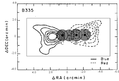
Fig. 1.— The ISO-LWS pointing positions are superimposed on the CO outflow map in B335. The cross and the squares indicate the position of the far-infrared source and of the three HH119 objects (A, B and C) respectively. The rectangular area outlines the region of the raster map.
