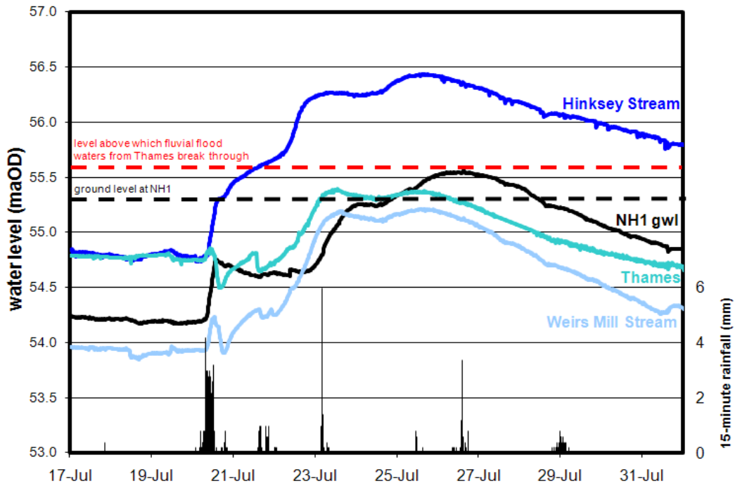
Figure 8 Fluvial flood water levels upstream of the Botley Road and interpolated groundwater levels at an urban location down-gradient of the Botley Road, Oxford during the July 2007 flood event. Also shown, 15-minute rainfall data, the threshold of the lowest property in the urban area down-gradient of the Botley Road and the level above which the flood waters upstream of the Botley Road would overtop. BGS © NERC 2011. 15-minute rainfall data were provided by the Environment Agency.
