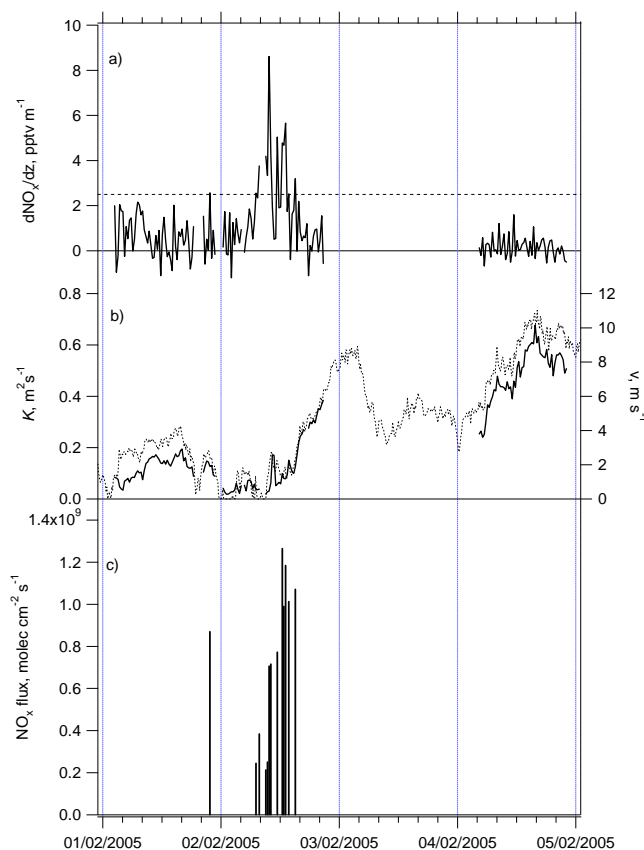
Fig. 4. (a) 20 min averaged NO x gradients ( \frac{\partial \text{NO}_x}{\partial z} ) estimated from the 1.5 and 6 m high inlets NO x measurements; the horizontal dashed line (2.5 pptv m -1 ) corresponds to the 2 \sigma precision of the gradient measurements; (b) 20 min averaged surface diffusivities ( K ) estimated from the friction velocities U_* at 4 m height (solid line, left-hand axis), and 10 min averaged wind speeds (dotted line, right-hand axis); (c) 20 min averaged NO x fluxes expressed as the product \frac{\partial \text{NO}_x}{\partial z} \times K , filtered for gradients less than 2.5 pptv m -1 detection threshold. NO x gradient were not measured during 3 February 2005 due to instrument downtime/maintenance.
