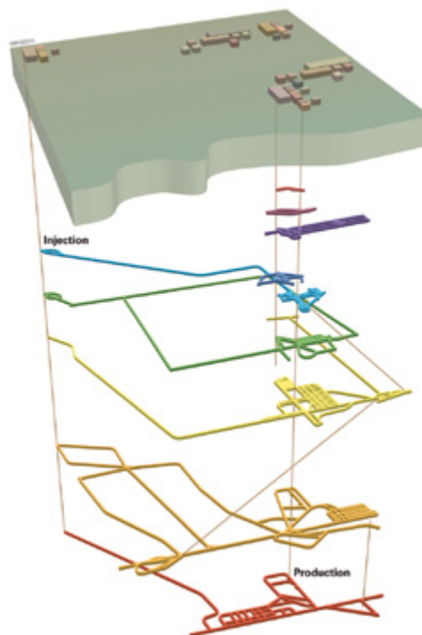
A 3D representation of a minewater-related ground source heat reservoir, at Heerlen in the Southern Netherlands (modified after Mine Water Project 2008; see www.minewaterproject.info ).
