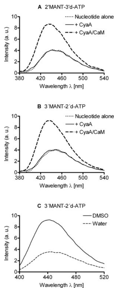
Fig. 4. Direct fluorescence of MANT nucleotides. The excitation wavelength was 350 nm, and emission was scanned from 380 to 550 nm. 100 nM nucleotide, 2.4 μM CyaA, and 2.4 μM CaM were added to cuvettes A and B in sequence. To mimic binding of the MANT group to a hydrophobic binding pocket, 3'MANT-2'd-ATP was directly excited in water plus dimethyl sulfoxide (DMSO) 30% (v/v) (C). Shown are superimposed recordings of a representative experiment. Similar data were obtained in five independent experiments. a.u., arbitrary unit.
