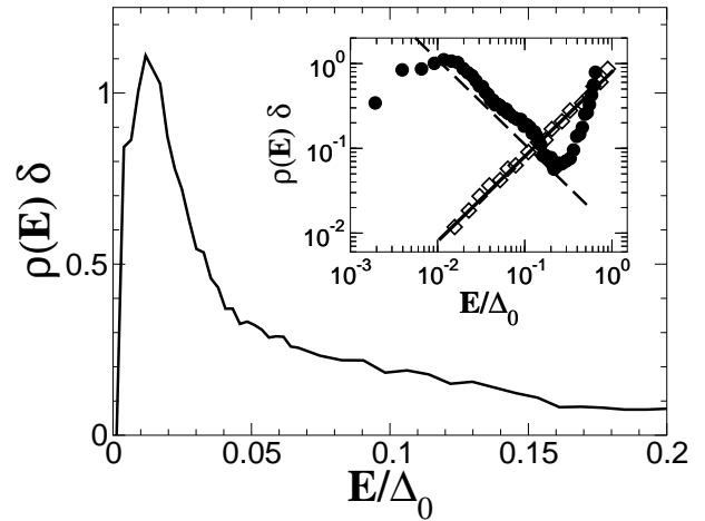
FIG. 2: Main plot: Low energy DoS for the d-wave Bogoliubov-de Gennes kicked rotator of Eqs. (2-4), L_x \times L_y = 256 \times 256 , \Delta_0 = 0.4 , E_F = 2\pi^2/5 , and K = 8 . Inset: Asymptotic of the density of states at low excitation energy for the same set of parameters, for long-wavelength disorder (quantum chaotic; black circles) and diffractive disorder as defined in Eq. (6) with N_H = 27 (quantum disorder; empty diamonds). The solid and dashed lines indicate a \propto E and \propto E^{-1} behavior respectively.
