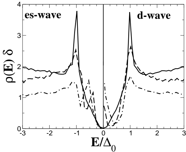
FIG. 1: Density of states for the d-wave (right) and extended s-wave (left) Bogoliubov-de Gennes kicked rotator defined by Eqs. (2-4), and parameters L_x \times L_y = 128 \times 128 , \Delta_0 = 0.4 , E_F = 2\pi^2/5 , and K = 0 . (solid lines), 2. (dashed lines) and 8. (dotted-dashed lines).
