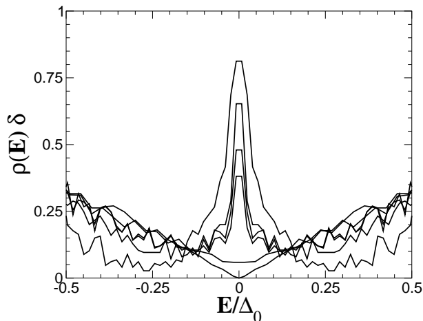
FIG. 3: Low energy DoS for the d-wave Bogoliubov-de Gennes kicked rotator with decreasing disorder range as defined in Eqs. (2), (4) and (6), with L_x \times L_y = 256 \times 256 , \Delta_0 = 0.4 , E_F = 2\pi^2/5 , K = 8. , and N_H = 1, 3, 5, 7, 17 , and 27 (from top to bottom).
