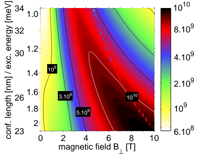
FIG. 2: (Color online) Orbital relaxation rate (the sum of the deformation and piezoelectric contribution) in a single quantum dot as a function of magnetic field and the confinement length l_0 / the confinement (excitation) energy E_0 . The rate is given on the logarithmic scale in the units of s^{-1} . The solid lines represent equal relaxation rates (equipotential lines). The granular structure in the figure is an artifact of the limited data resolution.
