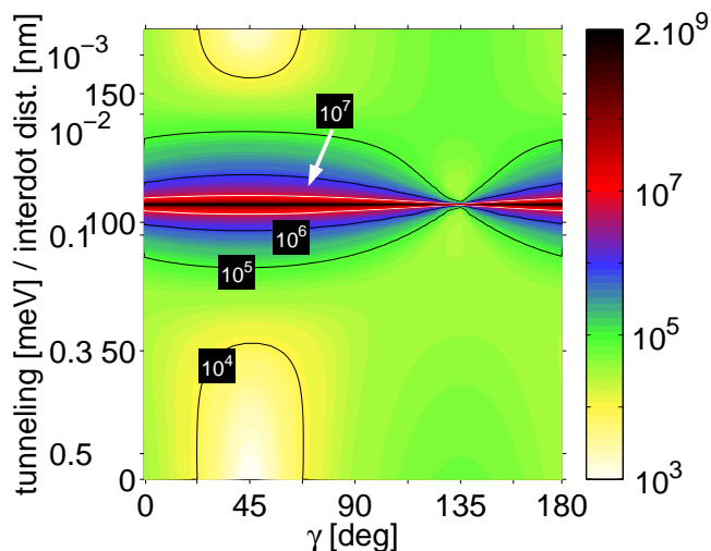
FIG. 9: (Color online) Spin relaxation rate in a double dot as a function of the orientation of the in-plane magnetic field and tunneling energy for B = 5 T, for [001] growing direction. The dot orientation is given by \delta = \pi/4 . A small asymmetric term is added into the confinement potential (an electric field of 10^3 V/m in y direction is applied in on one of the dots). By this, the easy passage is turned into a weak passage – compare with Fig. 4 in Ref. 37.
