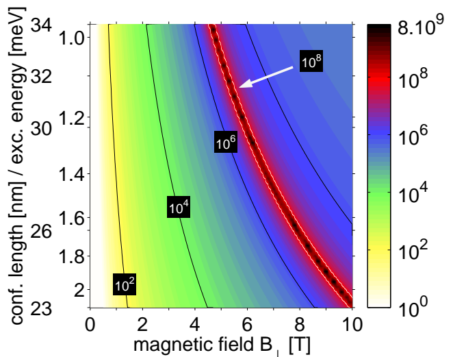
FIG. 3: (Color online) Spin relaxation rate in a single quantum dot as a function of magnetic field and the confinement length l_0 / the confinement energy E_0 . The rate is given on the logarithmic scale in the units of s^{-1} . The solid lines represent equirelaxation lines.
