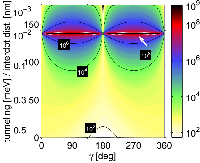
FIG. 7: (Color online) Spin relaxation rate as a function of \gamma and the tunneling energy for B_{\parallel} = 1 T, for [110] growing direction. The dot orientation is given by \delta = \pi/2 . The relaxation rate is given in logarithmic scale in the units of s^{-1} .
