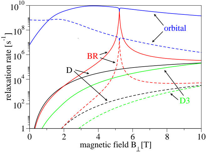
FIG. 1: (Color online) Orbital and spin (labels D , BR , and D3 denote which spin-orbit interaction is present) relaxation rates in a single quantum dot, for the piezoelectric (solid) and deformation potential (dashed) phonons. The confining length is 32 nm. Anti-crossing of the unperturbed spin and orbital state occurs at B_{\perp} = 5.2 T.
