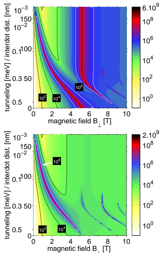
FIG. 6: (Color online) Spin relaxation rate as a function of perpendicular magnetic field for \gamma = 0^\circ and the interdot distance d / tunneling energy \delta E_t (at zero magnetic field only), for a confinement length 32 nm. The relaxation rate is given in logarithmic scale in the units of s^{-1} . The double dot is oriented along [100] ( \delta = 0^\circ ). The upper figure shows results when only the Bychkov-Rashba term is present in the Hamiltonian. In the lower figure, only the Dresselhaus terms are present.
