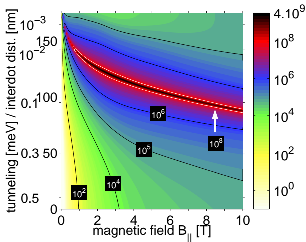
FIG. 4: (Color online) Spin relaxation rate in a double quantum dot as a function of in-plane magnetic field for \gamma = 0^\circ and the interdot distance d / tunneling energy \delta E_t , for a confinement length 32 nm. The relaxation rate is given on the logarithmic scale in the units of s^{-1} . The double dot is oriented along [100] ( \delta = 0^\circ ).
