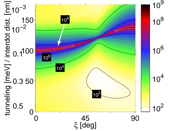
FIG. 8: (Color online) Spin relaxation rate as a function of \xi and tunneling energy for B = 1 T, for [110] growing direction. The dot orientation is given by \delta = \pi/2 . The relaxation rate is given in logarithmic scale in the units of s^{-1} .
