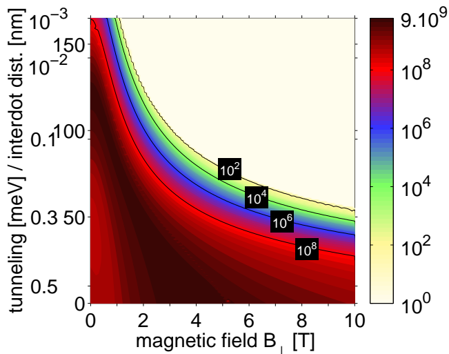
FIG. 5: (Color online) Orbital relaxation rate in a double quantum dot as a function of in-plane magnetic field for \gamma = 0^\circ and the interdot distance d / tunneling energy \delta E_t , for a confinement length 32 nm. The relaxation rate is given on the logarithmic scale in the units of s^{-1} . The double dot is oriented along [100] ( \delta = 0^\circ ).
