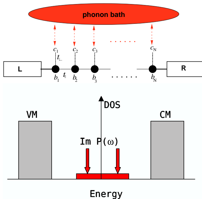
FIG. 1: Schematic representation of the DNA molecular wire in contact with a phonon bath (upper panel) and of the corresponding density of states (lower panel). In the absence of the phonon bath, valence (VM) and conduction (CM) manifolds are separated by a gap. Upon coupling to the environment, a new set of states emerge within the gap. Though strongly damped by the dissipative coupling, they yield a finite density of states and eventually lead to a conductance enhancement with increasing temperature.
