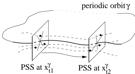
FIG. 5: Sketch of the PSS as it is shifted along the periodic orbit \gamma (solid line). Three pieces of the time-reversed orbit \gamma^i are represented by dashed lines. If the PSS moves with the flow in phase space from \mathbf{x}_{t_1}^\gamma to \mathbf{x}_{t_2}^\gamma all intersection points of the PSS with \gamma^i change their positions according to the linearized equations of motion (20). Note that not only \gamma^i but also \gamma itself could come close to \mathbf{x}_{t_1}^\gamma at a later time. However, we have not include this in the sketch above.
