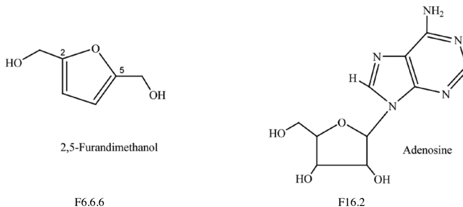
FIGURE 5. Chemical structures of F6.5.5 and F16.2 isolated from Fusarium proliferatum crude extract
