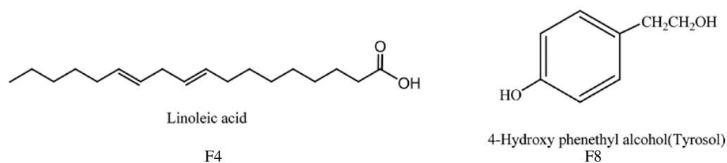
FIGURE 4. Chemical structures of F4 and F8 isolated from Fusarium proliferatum crude extract
