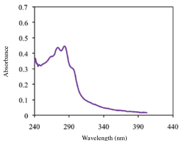
FIGURE 2. UV spectrum of Fusarium proliferatum extract
