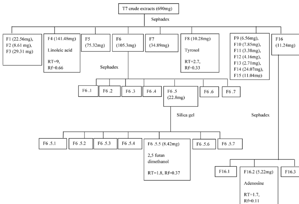
FIGURE 1. Analytical scheme for purification of metabolites from Fusarium proliferatum crude extract
