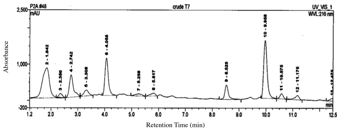
FIGURE 3. HPLC chromatogram on Fusarium proliferatum crude extract
