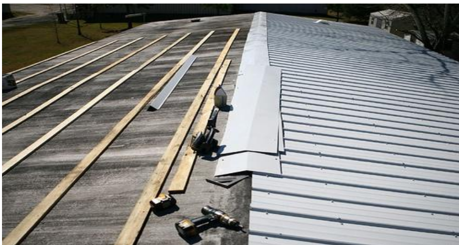
Figure 10: Metal roofing (Source: www.metalroofingtips.com )
