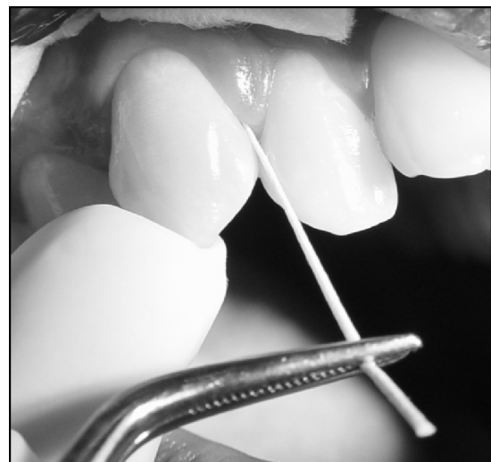
FIGURE 1. GCF sampling
