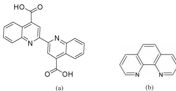
FIGURE 1. Structures of (a) 2,2'-biquinoline-4,4'-dicarboxylic acid and (b) 1,10-phenanthroline
