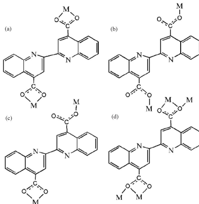
FIGURE 2. Coordination modes of 2,2'-biquinoline-4,4'-dicarboxylate ion: (a) bis-bidentate chelating (b) bis-monodentate (c) monodentate-bidentate chelating (d) bis-chelating-bridging tridentate (Dai et al. 2008)
