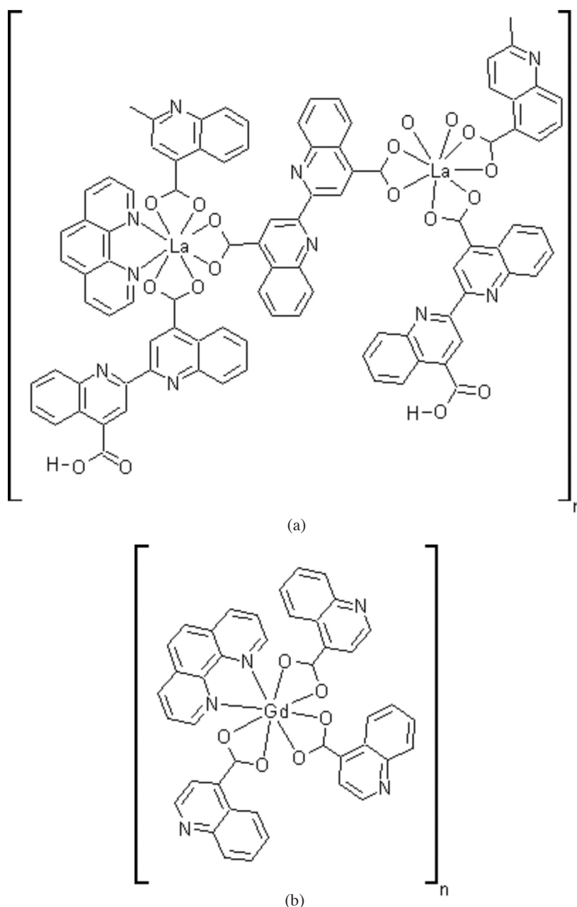
FIGURE 3. The suggested structures of (a) [La_2(Hbqda)_2(bqda)_2(phen)]_n [1] and (b) [Gd(bqda)_{1,5}(phen)]_n [2]
