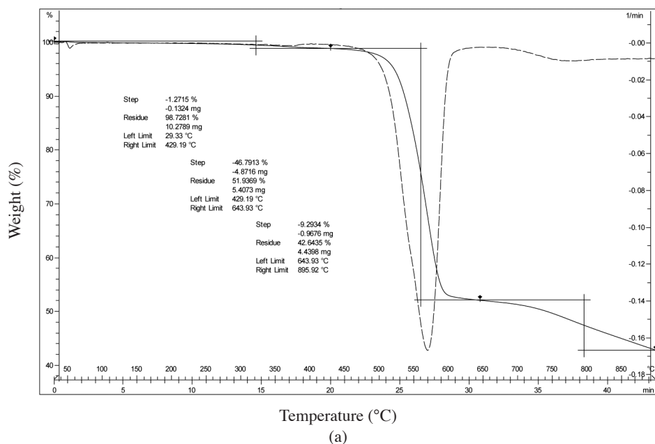
FIGURE 4. Thermograms of (a) [\text{La}_2(\text{Hbqda})_2(\text{bqda})_2(\text{phen})]_n [1] and (b) [\text{Gd}(\text{bqda})_{1.5}(\text{phen})]_n [2]
