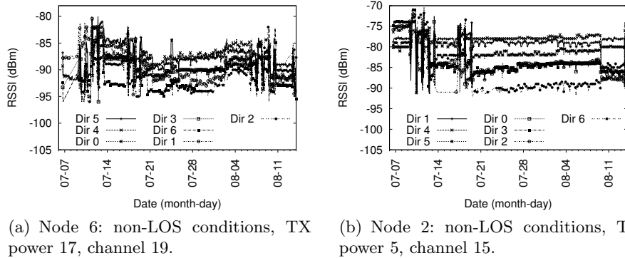
Fig. 4: Link performance along different antenna directions, compared to the omni-directional configuration. The best performing antenna direction changes over time.
