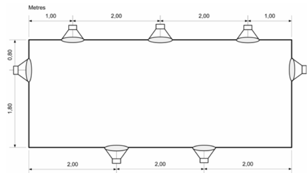
Figure 3. Loudspeaker placement on DigiWall
