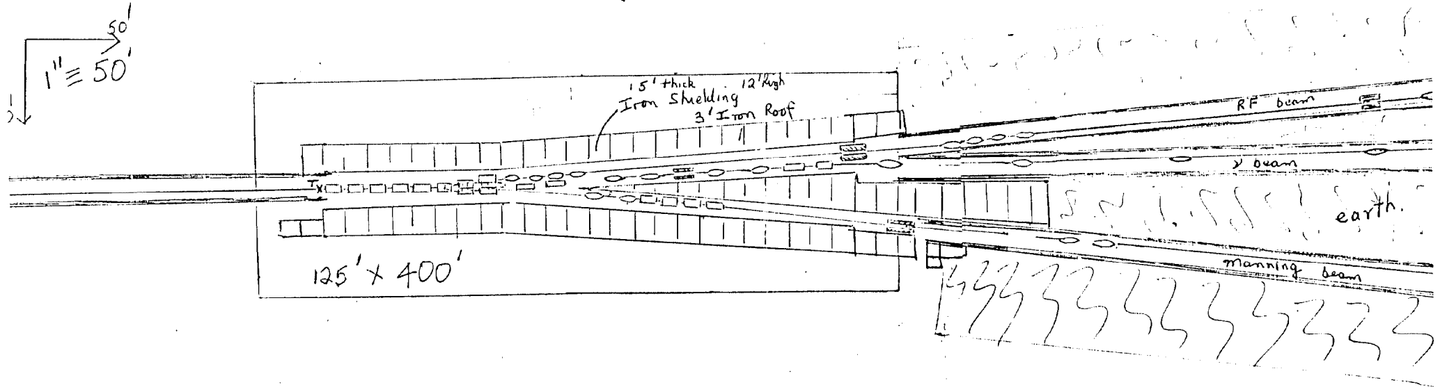
TARGET STATION C--PRELIMINARY LAYOUT OF BEAMS
