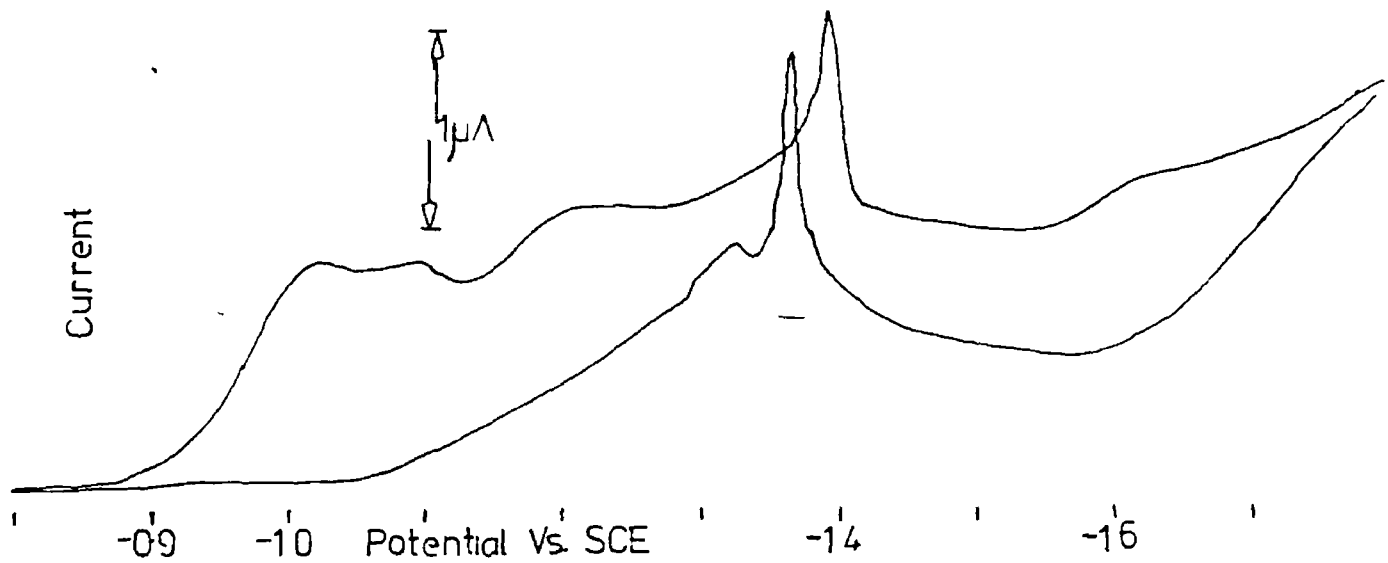
Fig. 33b Cyclic Voltammogram of OTC in 0.1M KCl, Scan Rate 50 mV/sec
