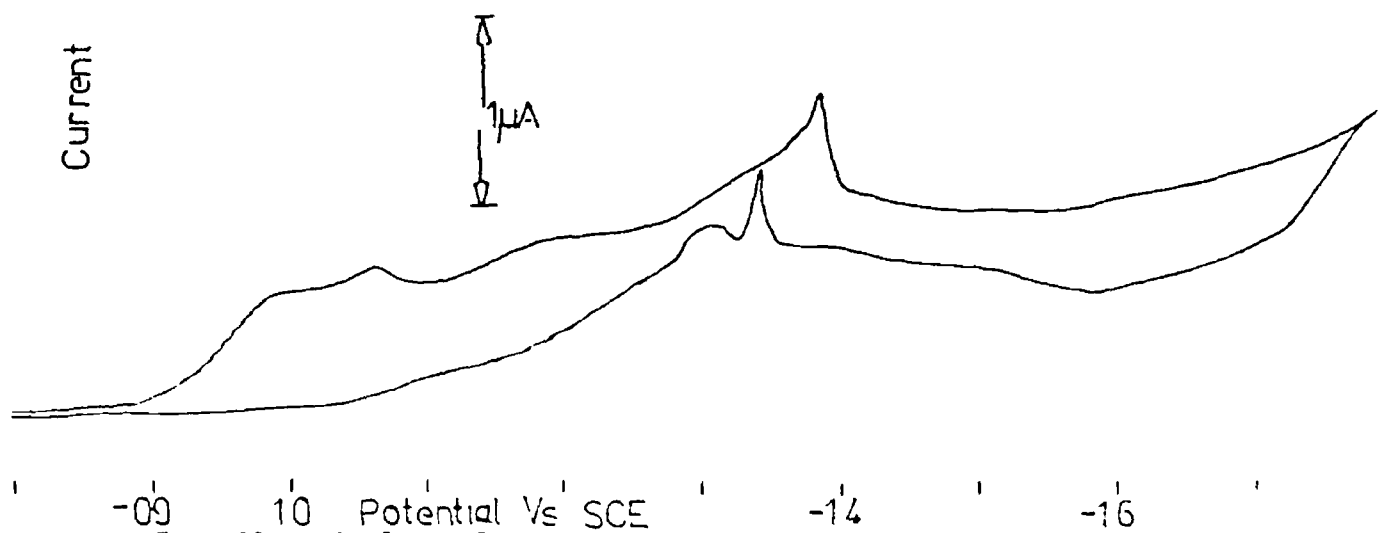
Fig. 33c Cyclic Voltammogram of OTC in 0.1M KCl, Scan Rate 20 mV/sec
