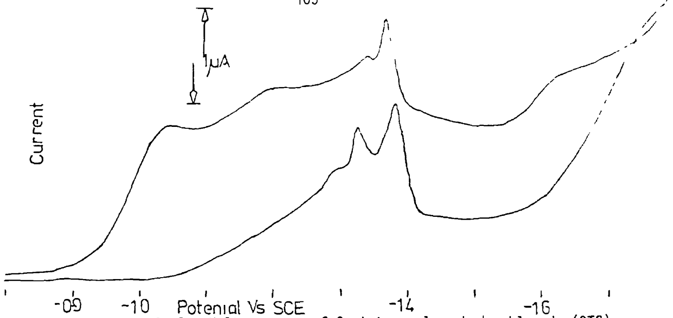
Fig. 33a Cyclic Voltammogram of Oxytetracycline hydrochloride (OTC) in 0.1M KCl, Scan Rate 100 mV/sec
