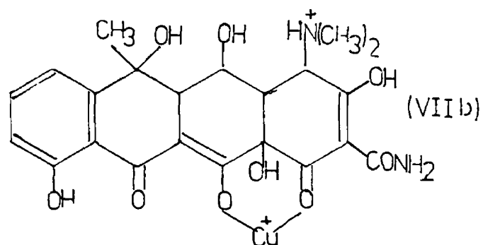
Fig. 15. Possible chelating sites of the Cu(II) ion to Oxytetracycline hydrochloride (BCD chromophore).
