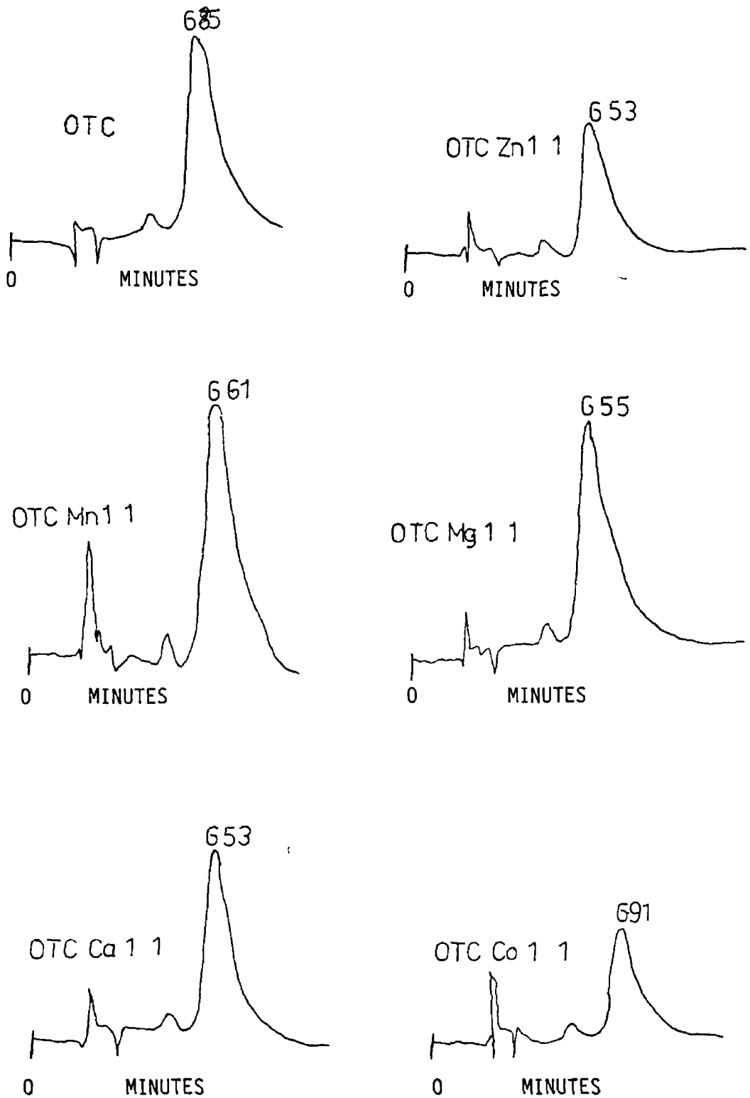
Fig. 34 Chromatograms of Oxytetracycline hydrochloride and its metal complexes. Column C_{18} Bondpak in mobile phase methanol-water 50:50 + 1 \times 10^{-5} M Oxytetracycline Hydrochloride, Ultraviolet detection at 280 nm, Flow Rate 1.5 ml/min.
