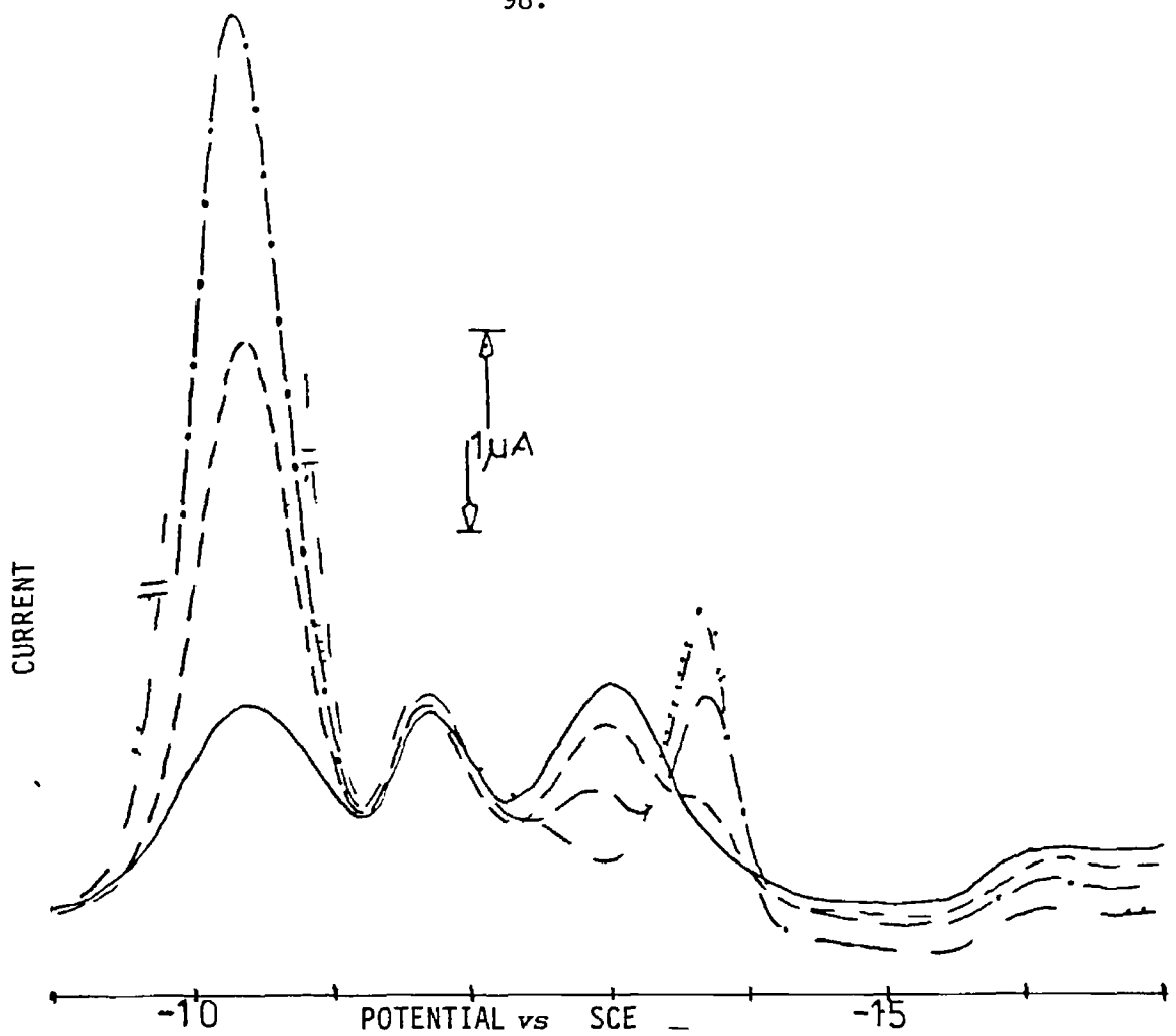
Fig. 30a Differential Pulse Polarograms of Oxytetracycline hydrochloride (OTC) (—), OTC Zn(II) 1:1 (----), OTC Zn(II) 1.2 (-·-·-), OTC Zn(II) 1.3 (···) and OTC Zn(II) 1.4 (-·-·-·-) in 0.1 M KCl.
