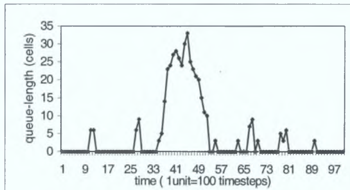
Figure 3.11. Queue-length of approach 4.
