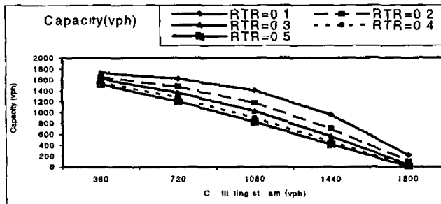
Fig 6 Capacity of a major-stream as for Fig 5a for rational driver behaviour
