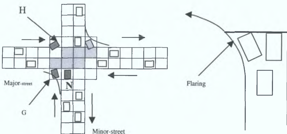
Figure 3.6 Intersection with flaring.
