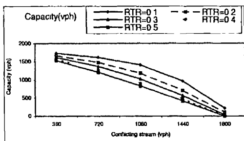
Fig 6 Capacity of a major street in situation of Fig 5a for rational driver behaviour
