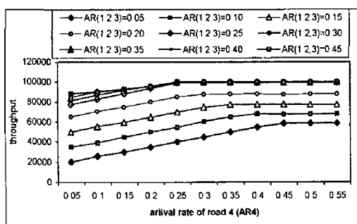
Fig 2 Throughputs vs arrival rates (AR)
