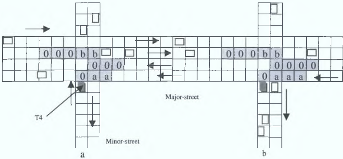
Figure 4.6. RT vehicle from a minor street: (a) rational behaviour and (b) conservative behaviour.
