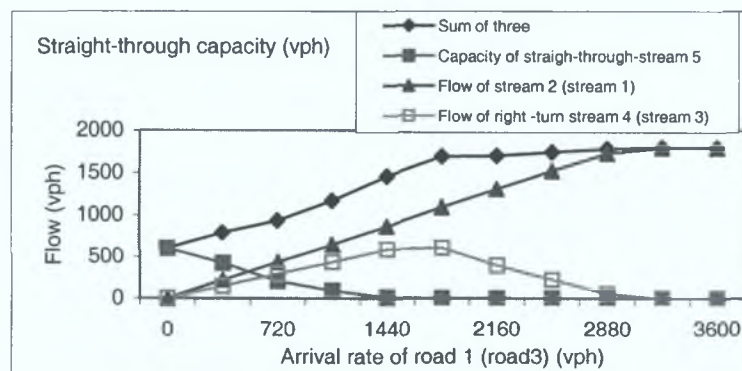
Figure 4.14. Minor street ST capacity
