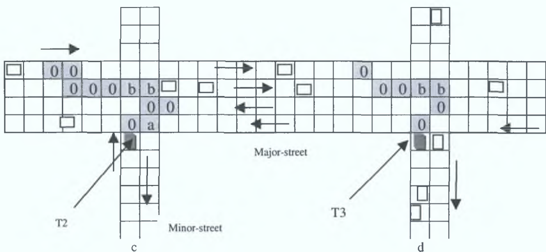
Figure 4.5. ST vehicle from a minor street: (c) urgent behaviour, and (d) radical behaviour
