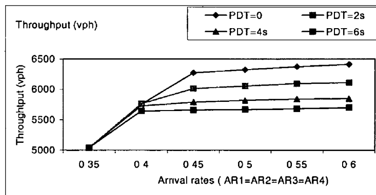
Figure 6 10 Throughputs vs PDT form Model B
