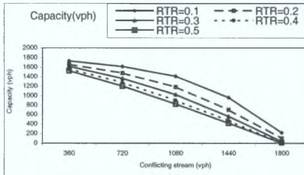
Figure 3.10 Capacity of a major-street in situation of Figure 3.9(a) for rational driver behaviour
