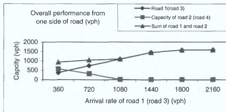
Figure 3.7. Overall performance of intersection
