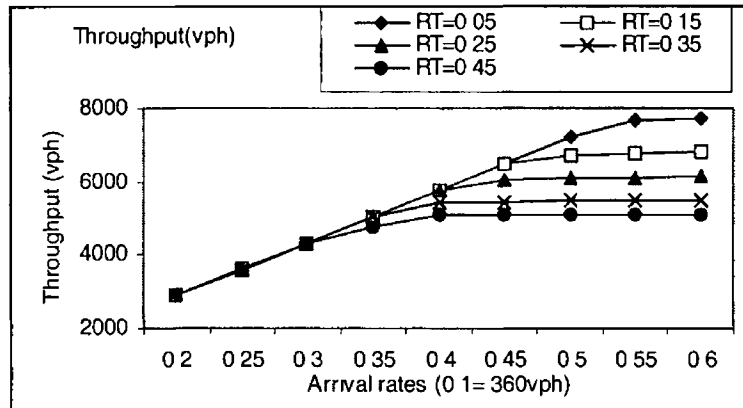
Figure 6 6 Throughput vs RTR rate for Model B
