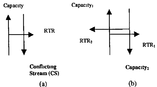
Fig 5 Traffic configurations of shared lane on the major streams
