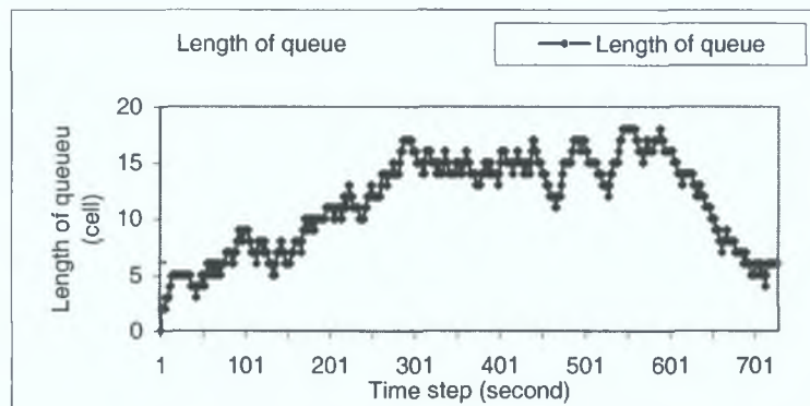
Figure 4.17. Queue-length of road 4
