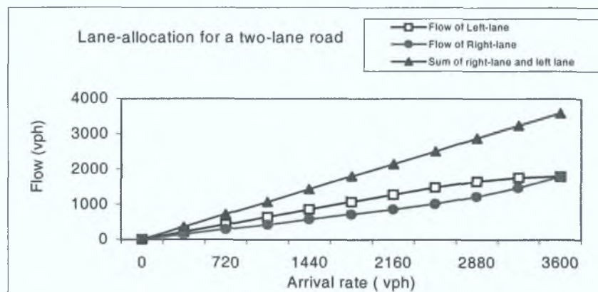
Figure 4.3 A lane-allocation pattern of RTR < 0.4 and LTR \leq 0.5 if there is no queue on the right-lane.
