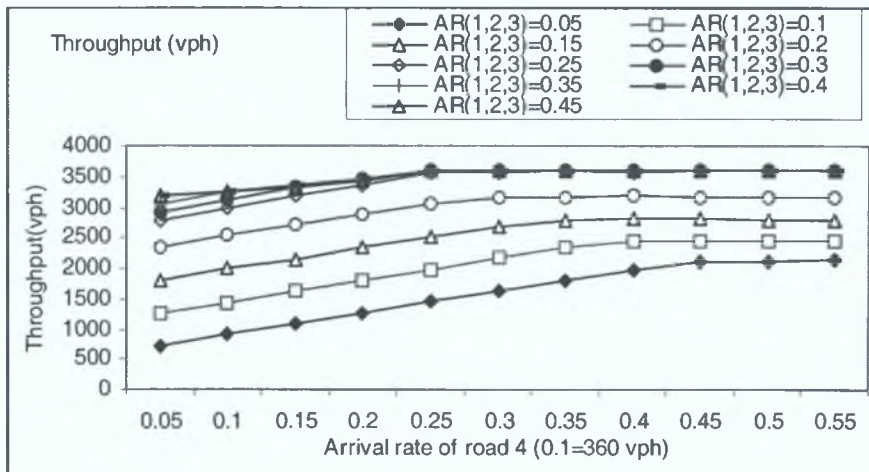
Figure 5.6: Throughputs vs. arrival rate.
