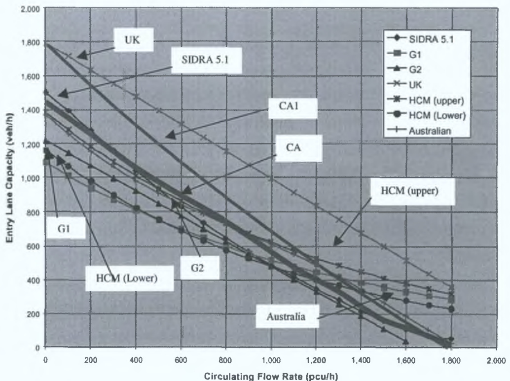
Figure 5.10: A comparison of roundabout methodologies
