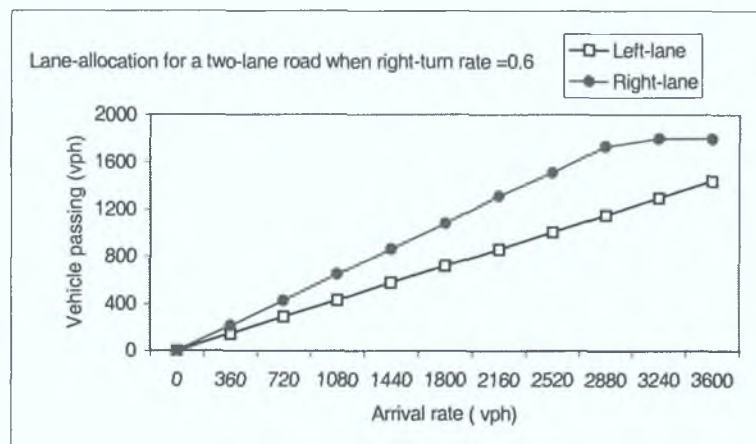
Figure 4.4. A lane-allocation pattern, when the RTR =0.6.
