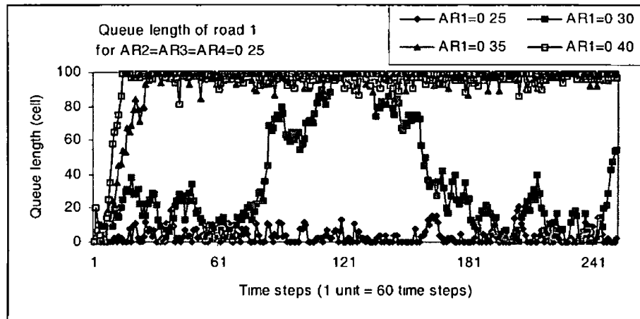
Figure 6.7 Queue-length of road 1 varied with AR_1 for Model A AR_1 increases from 0.2 to 0.4 when AR_2=AR_3=AR_4 = 0.25
