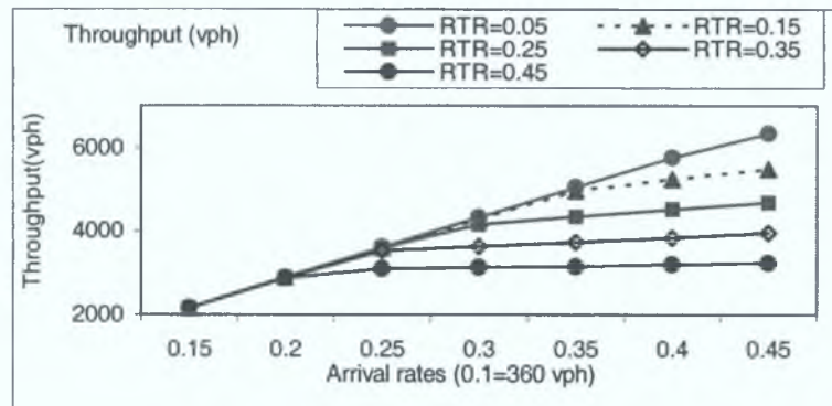
Figure 6.5 Throughputs change vs. right-turning rate for Model A
