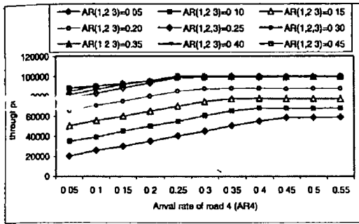
Fig 4 Throughputs vs arrival rates (AF)
