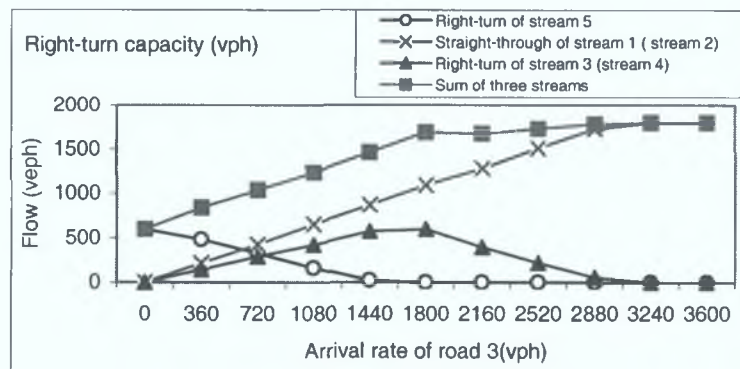
Fig 4.13 Minor street RT capacity
