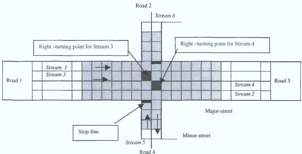
Figure 4.2. The intersection area where interactions between the vehicles occur
