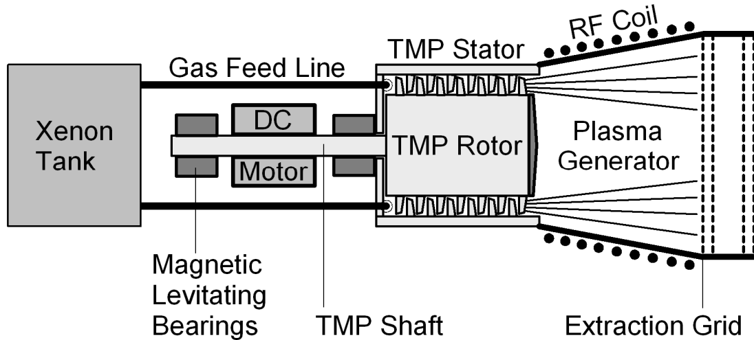
Fig. 1. Schematic diagram of the proposed turbomolecular pumping stage in an RF ion thruster.
