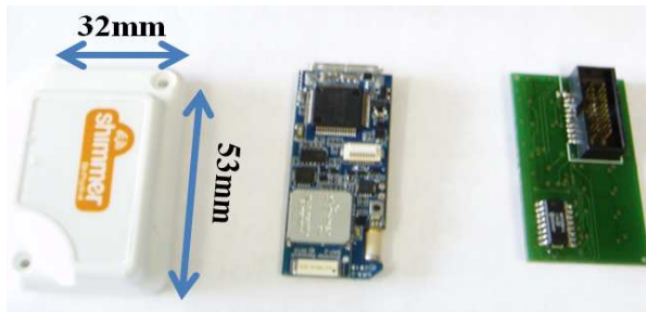
Figure 3. Left to right, casing, the main board and expansion board
