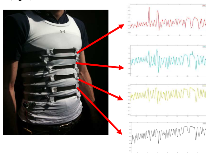
Figure 1. Respiratory shirt showing streams from several sensors.
