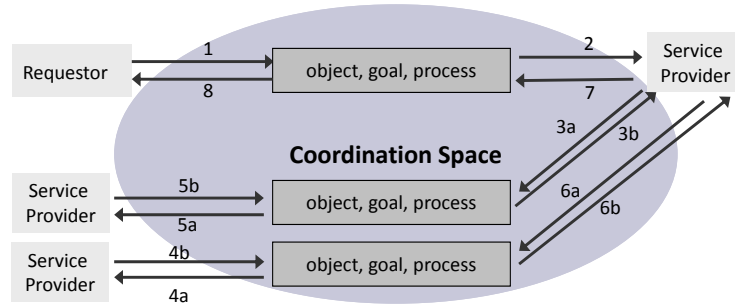
Figure 4 Abstract Coordinated Process of Requests
