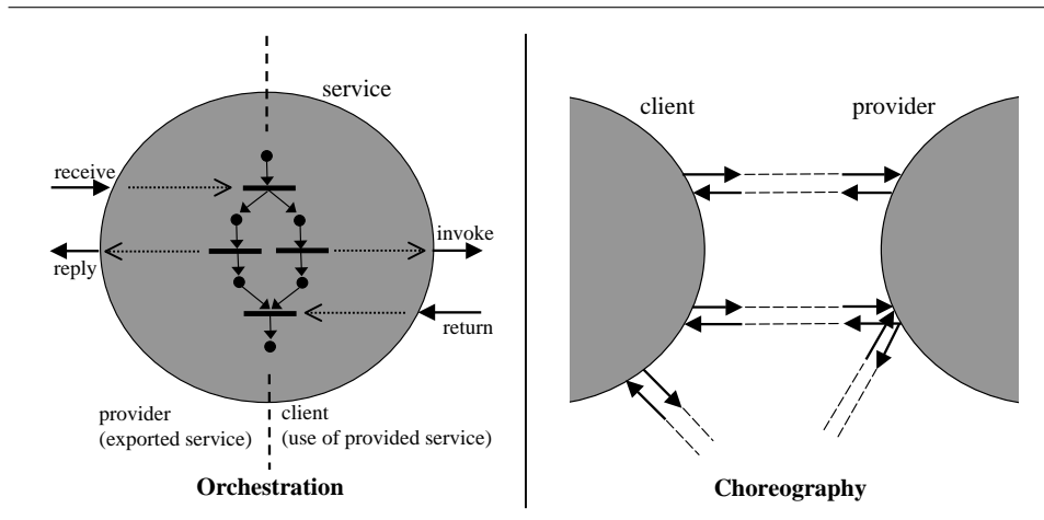
Fig. 5. Principles of Orchestration and Choreography.
