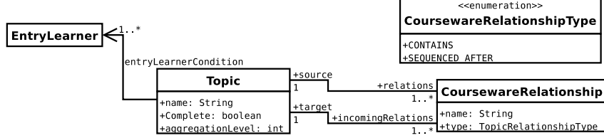
Figure 1: CAVIAr courseware metamodel excerpt
