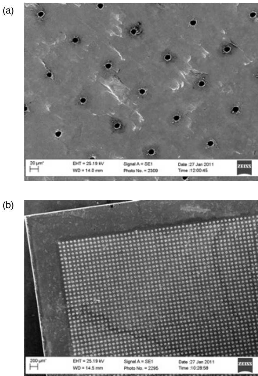
Figure 7.1 - SEM images of (a) \sim 10 \mu\text{m} feature size laser drilled holes on stainless steel foil, (b) wide field view of mask array.
