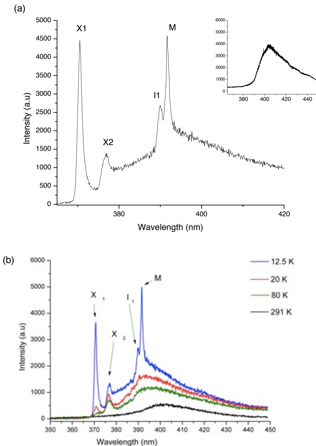
Figure 5.17 - Low-temperature PL measurement for CuCl-KCl melt produced sample (a) at 12.5 K with expected excitonic features I_1 and M biexciton and (b) formation of peaks as temperature decreases. Inset for (a) shows the room temperature PL data for comparison.
