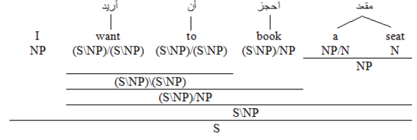
Figure 1: An Arabic sentence and its aligned English translation along with CCG derivation tree assigned to the English sentence.
