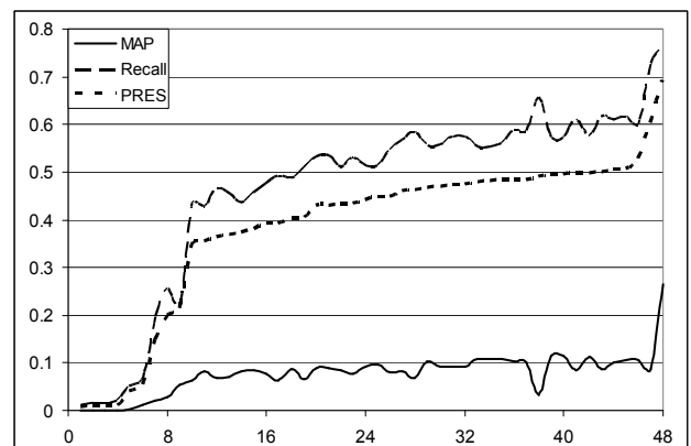
Figure 5. MAP/Recall/PRES for 48 submissions in CLEF-IP 2009 sorted by PRES
