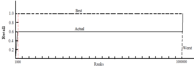
Figure 2. Illustration of how R_{norm} curve behaves with big collection of documents
