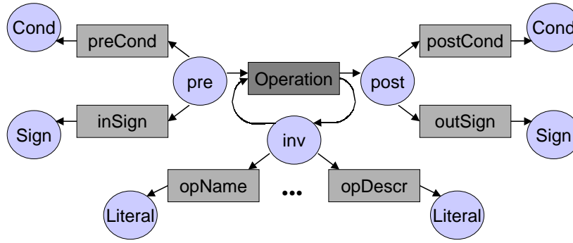
Fig. 3. Software Development Ontology based on Transitional Roles (Operation) and Descriptive Roles (preCond, inSign, etc.).
