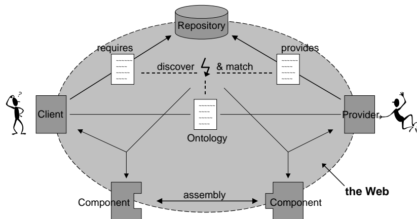
Fig. 1. Web-based Component Development Lifecycle based on Discovery/Matching and Assembly.
