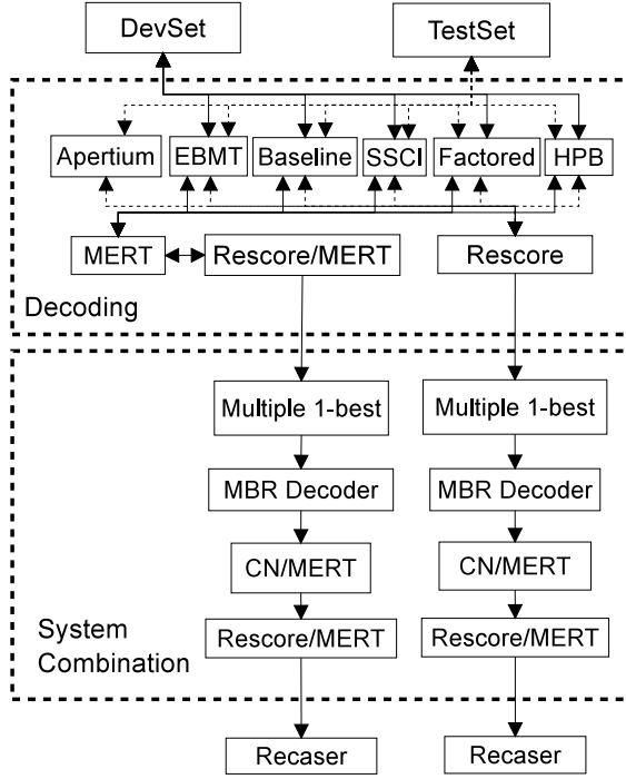
Figure 1: System Framework.
